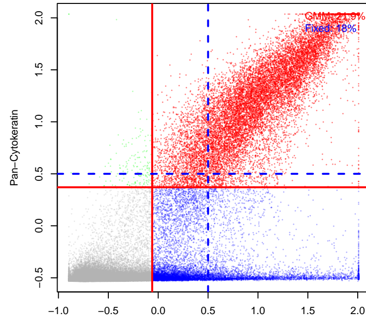
NYU1306_without_cd4_14_11c CD3e vs Pan-Cytokeratin
