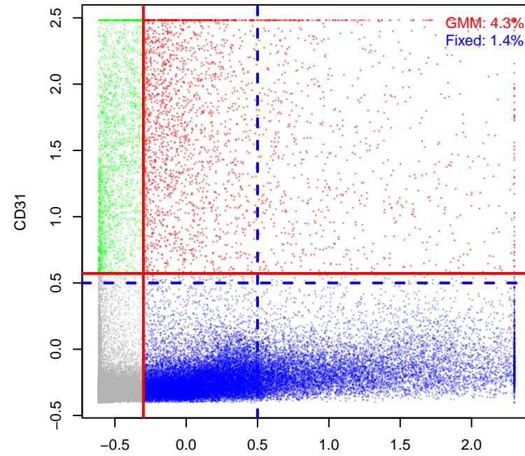
NYU1306_without_cd4_14_11c CD45 vs CD31
