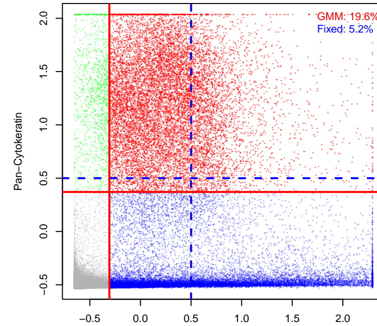
NYU1306_without_cd4_14_11c CD68 vs Pan-Cytokeratin
