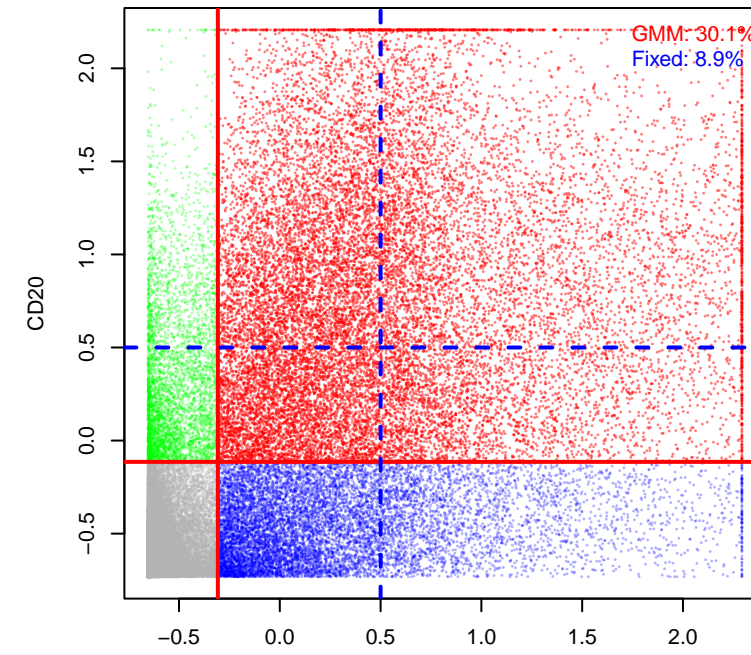
NYU1306_without_cd4_14_11c CD68 vs CD20
