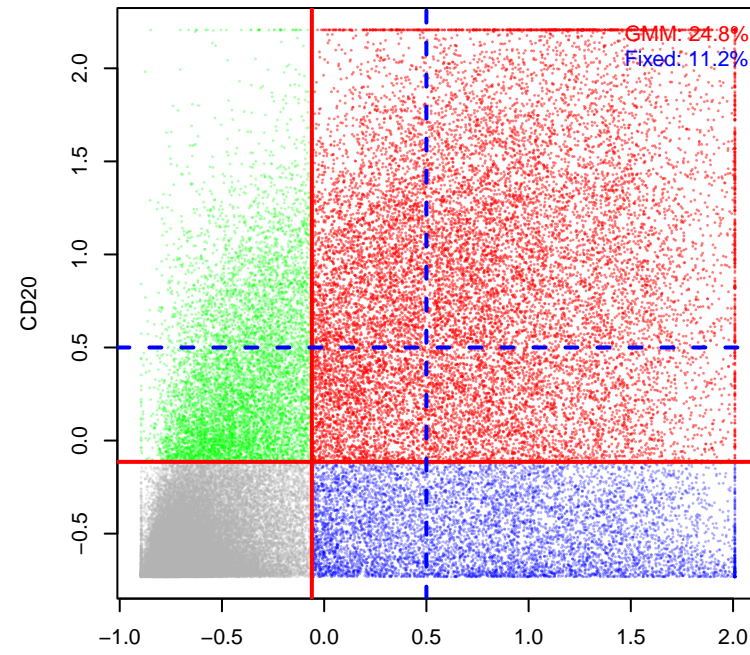
NYU1306_without_cd4_14_11c CD3e vs CD20
