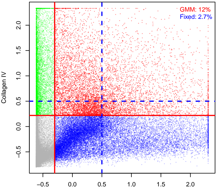
NYU1306_without_cd4_14_11c CD45 vs Collagen IV
