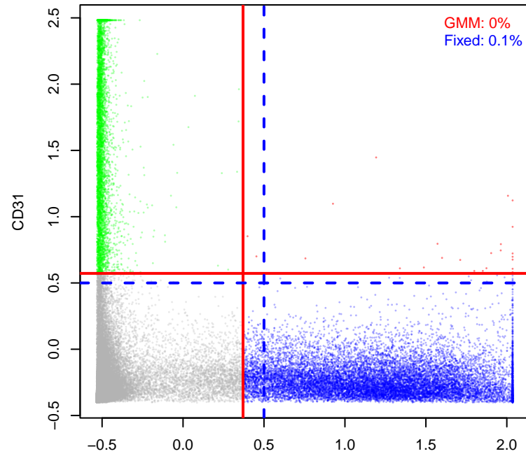
NYU1306_without_cd4_14_11c Pan-Cytokeratin vs CD31
