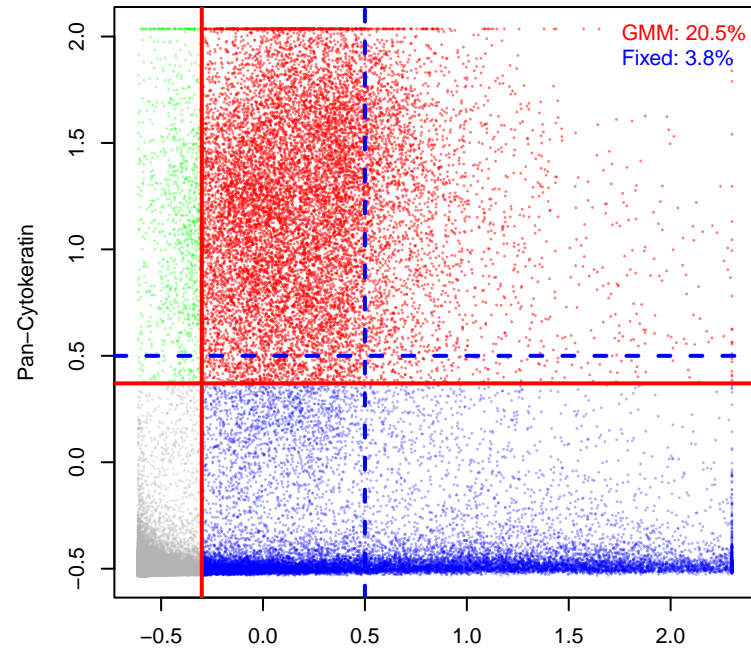
NYU1306_without_cd4_14_11c CD45 vs Pan-Cytokeratin
