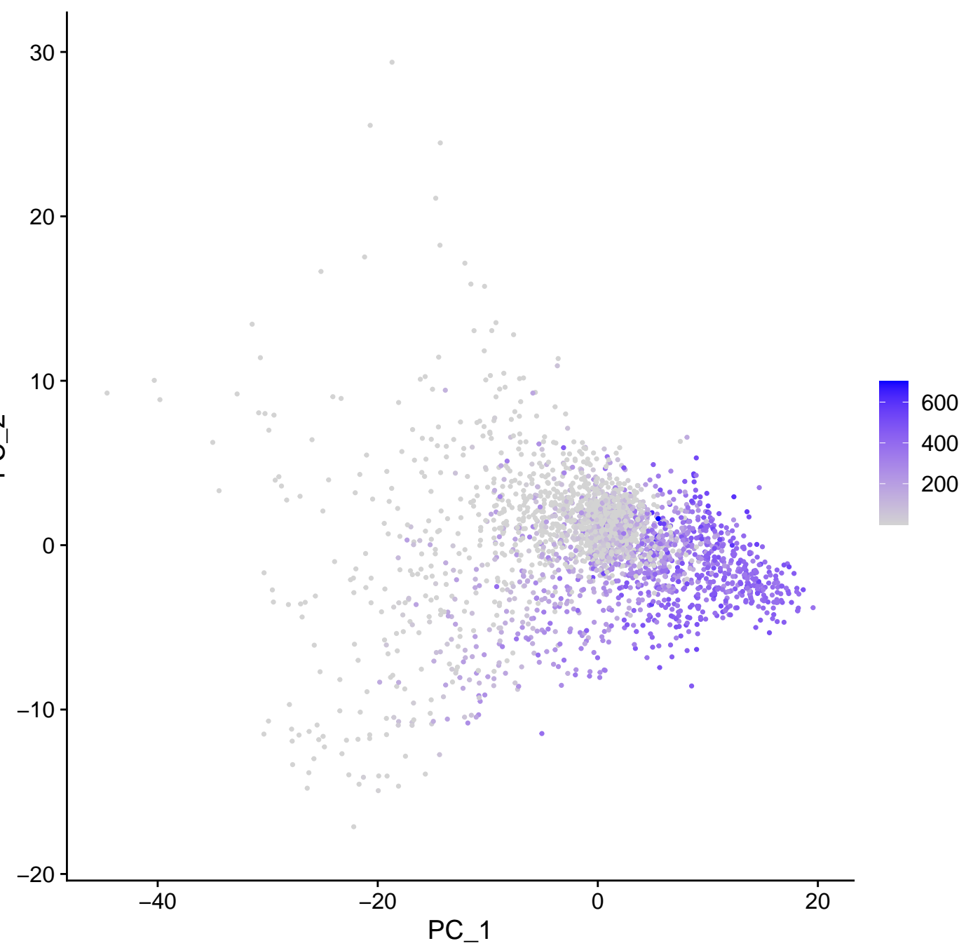
COL1A1
