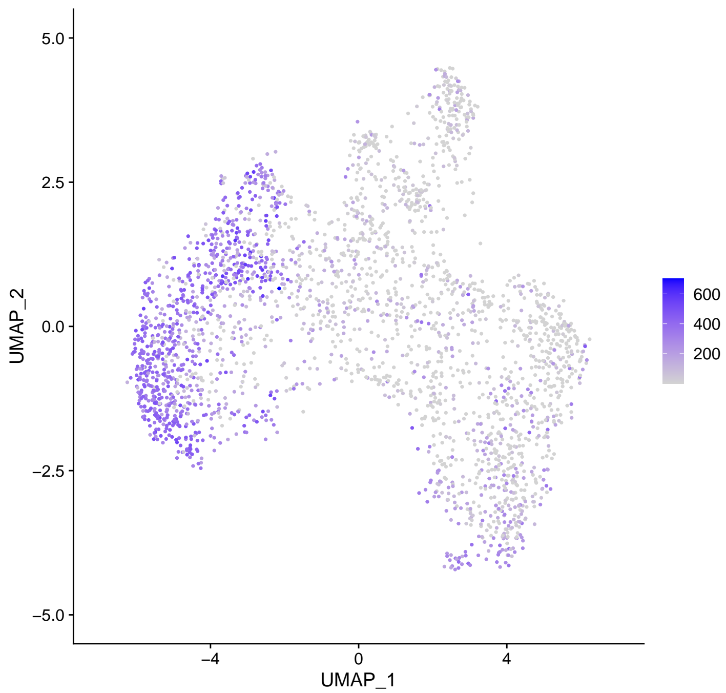
COL1A1
