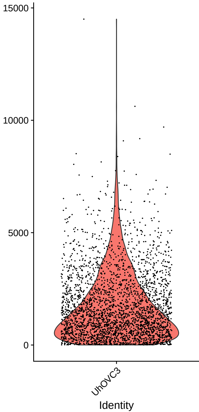
nCount_Spatial
