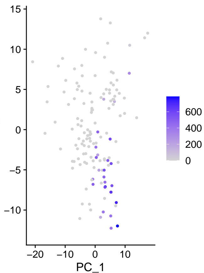
m_COL4A3BP
