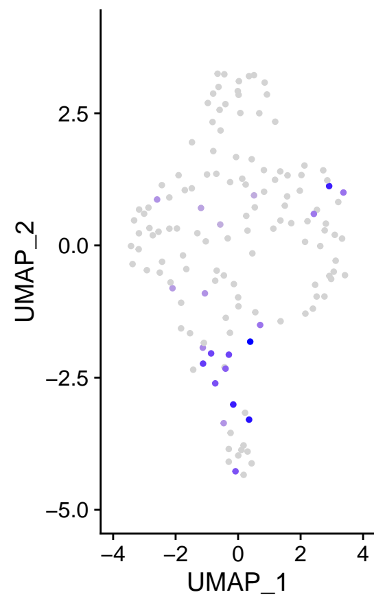
m_KRT18
