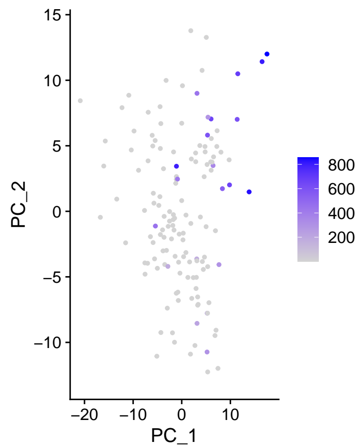
m_KRT18
