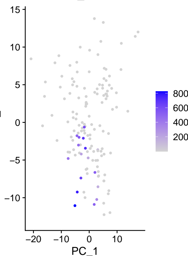
m_S100A6
