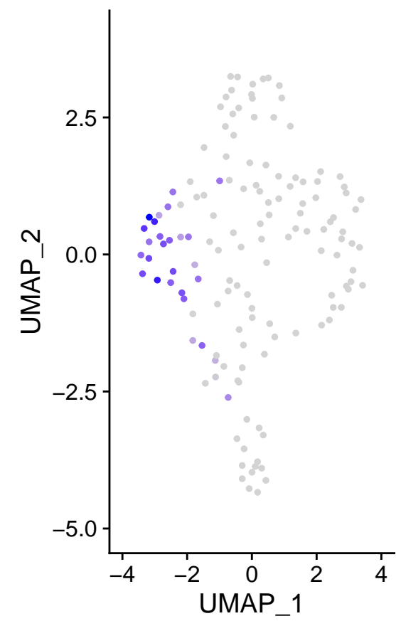
m_COL4A3BP
