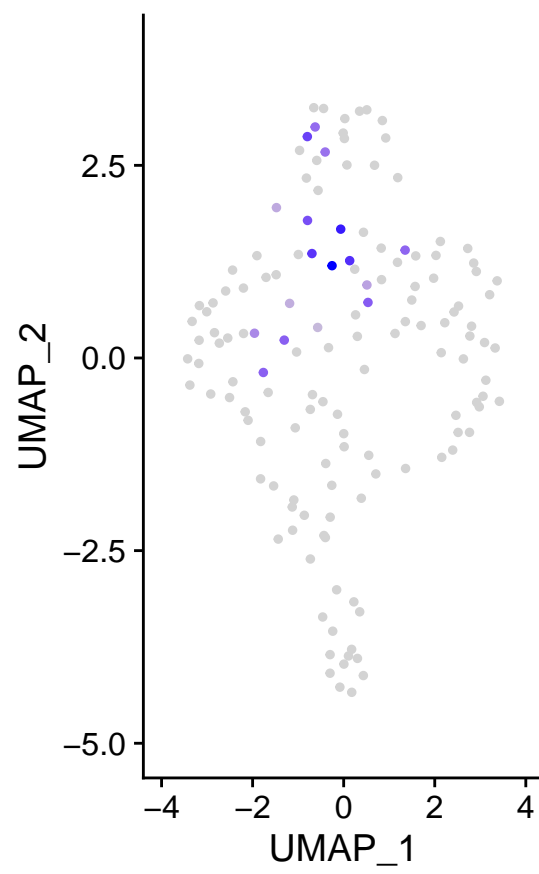
m_S100A6
