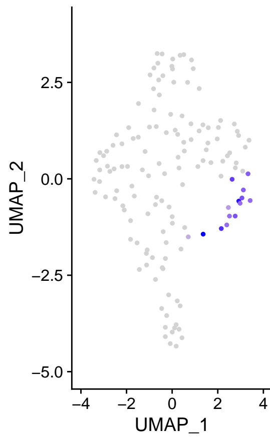
m_S100A6
