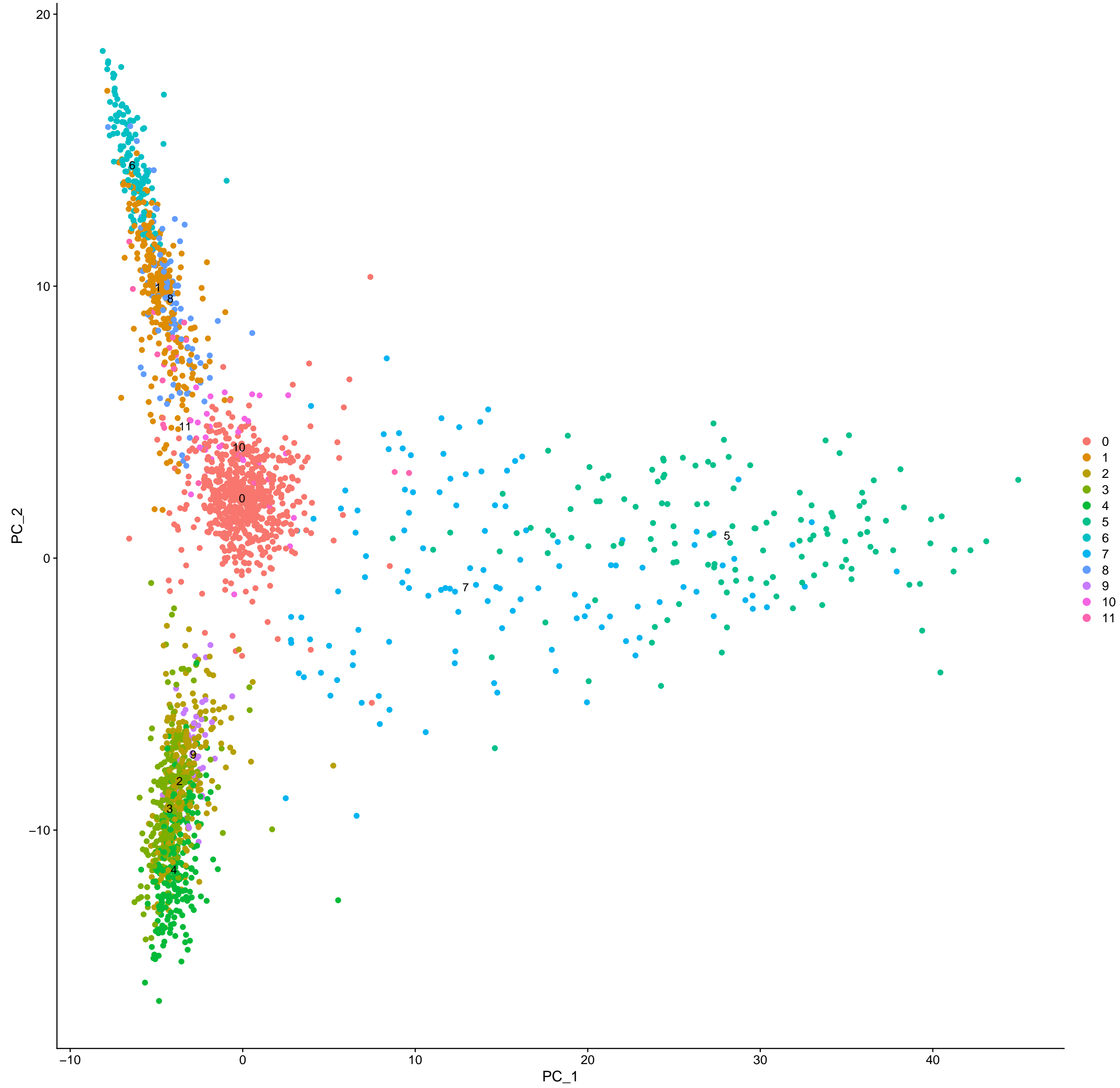
cluster
