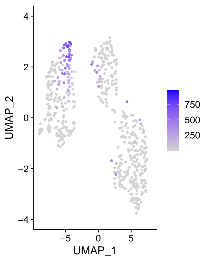
m_IFI27
