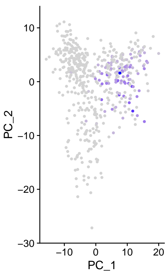
m_HSPA1A
