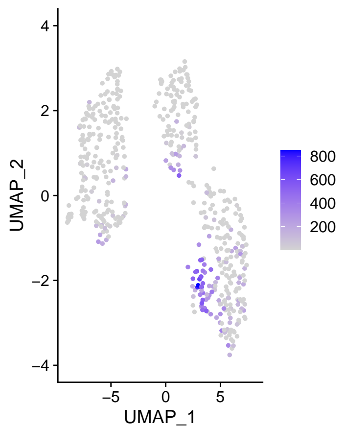
m_HAMP
