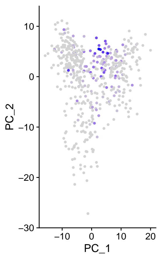
m_TUBA1B
