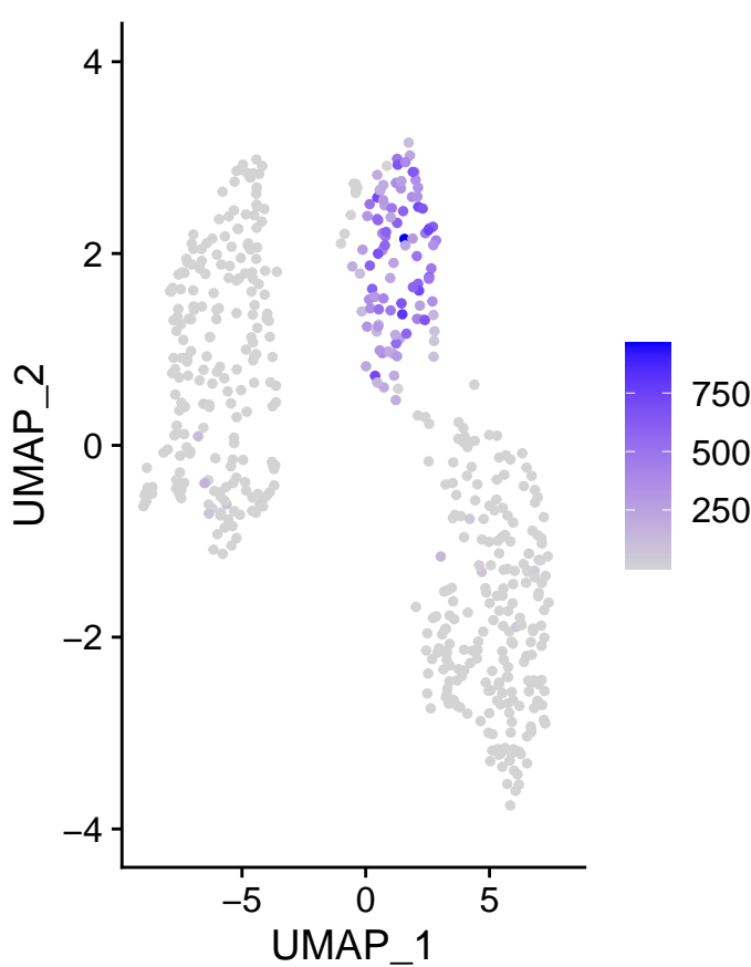
m_HSPA1A
