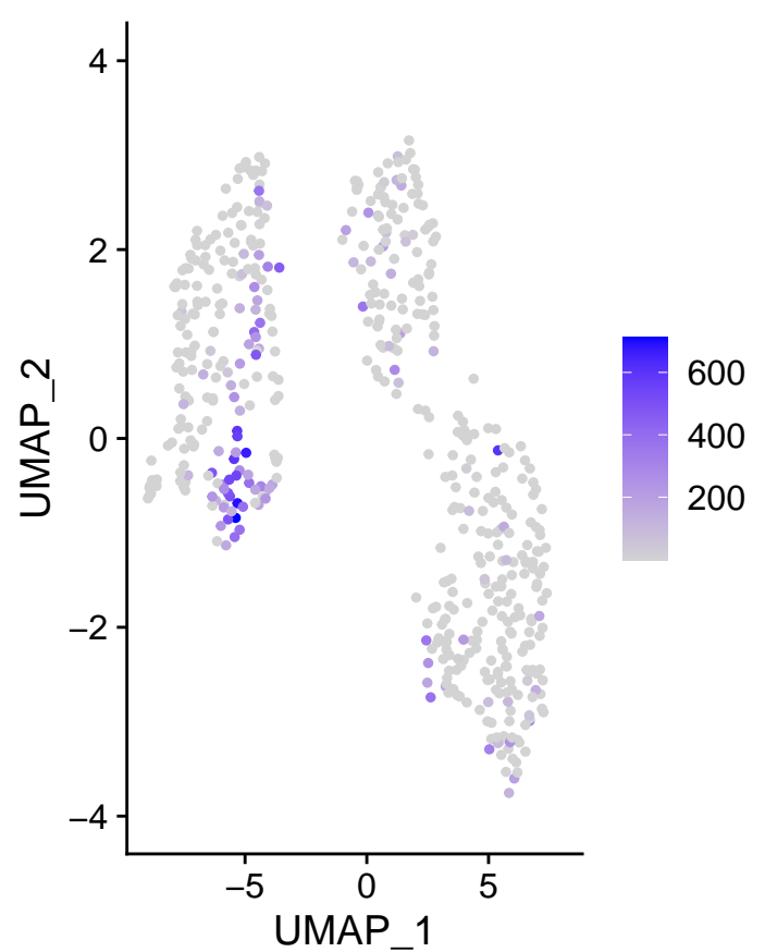
m_TUBA1B
