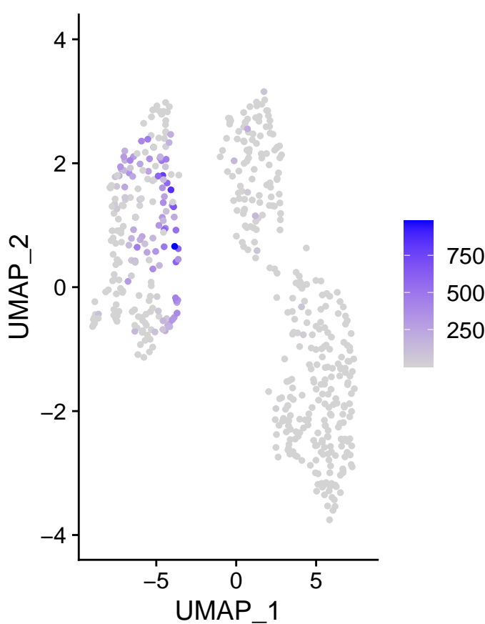
m_HSPA1A
