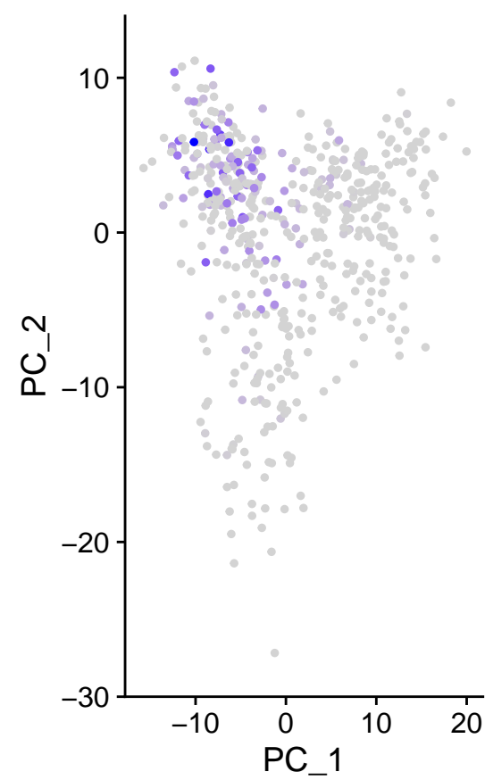
m_HAMP
