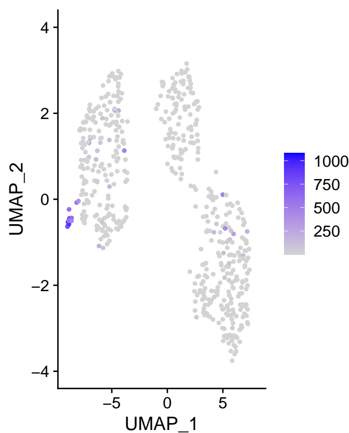
m_TUBA1B
