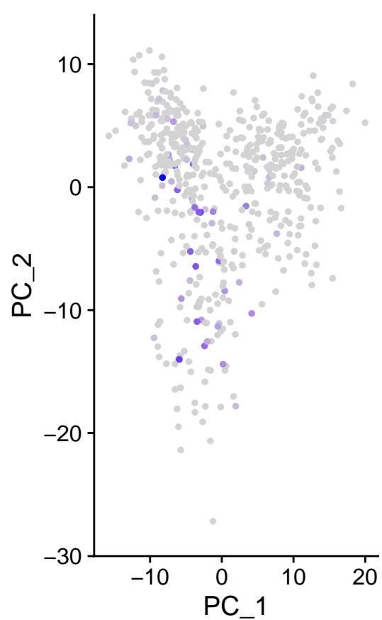
m_IFI27
