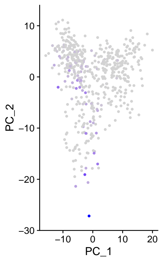
m_CYP3A4
