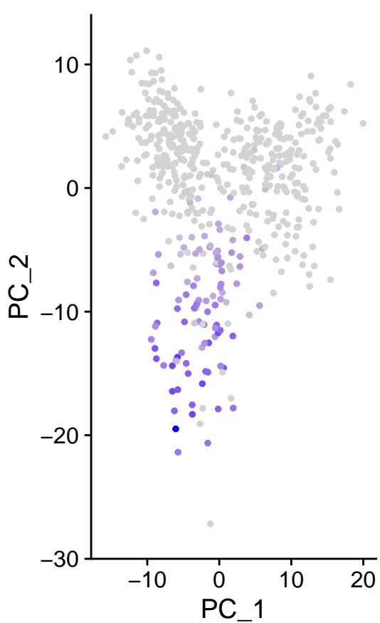
m_HSPA1A
