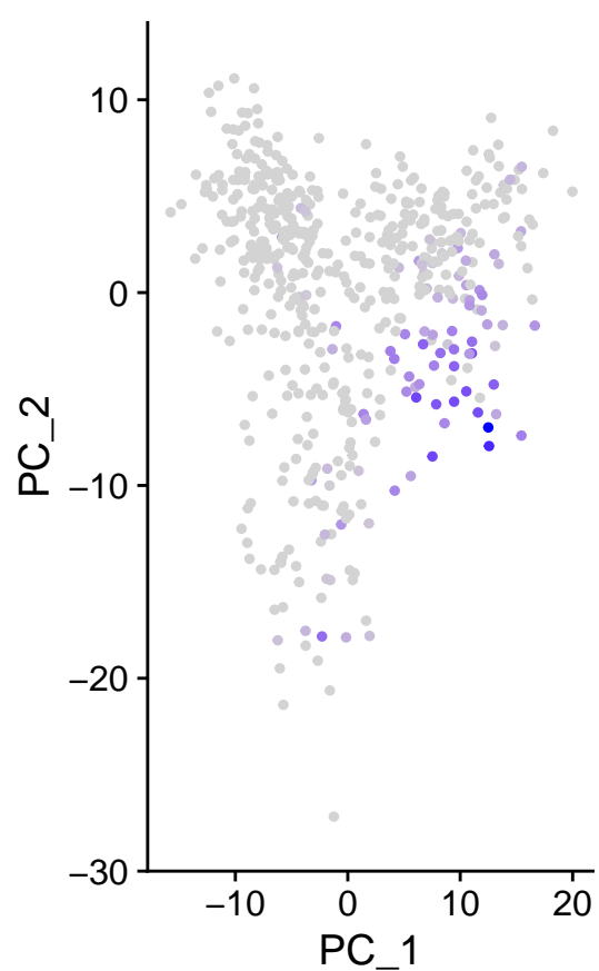
m_IFI27
