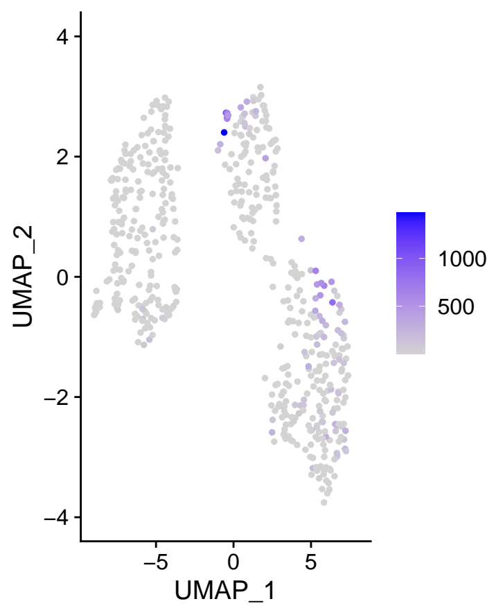
m_CYP3A4
