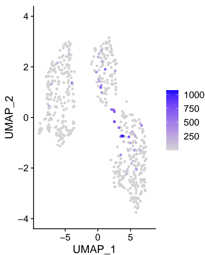
m_IFI27
