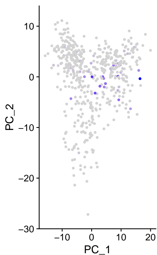
m_TUBA1B
