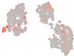
Cycle
