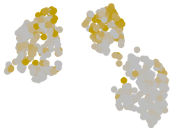
Interferon
