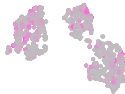
Glandular
