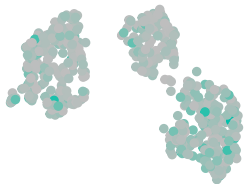
cEMT
