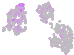
Squamous
