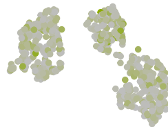
Hypoxia
