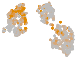
Stress
