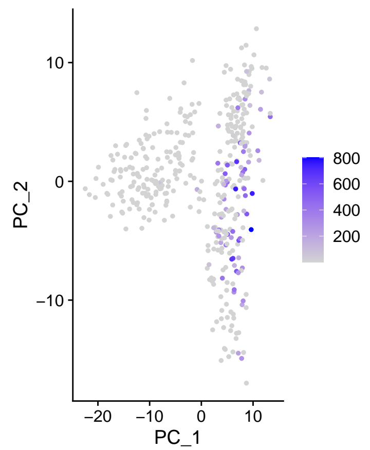
m_RND3
