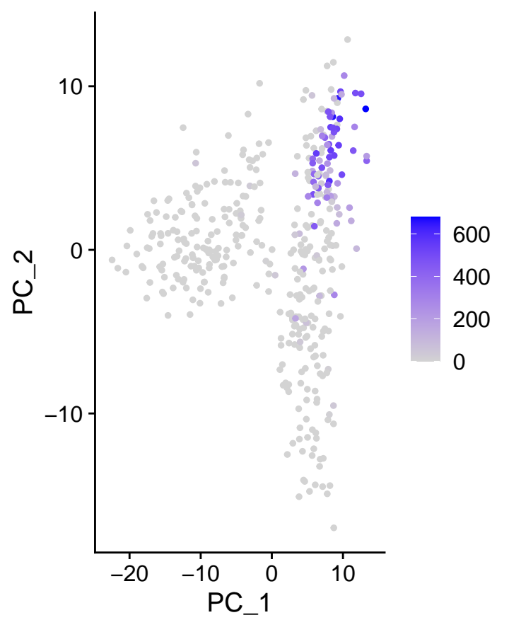
m_FBXL20
