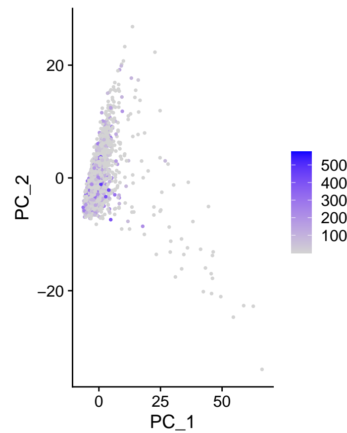
m_IGFBP7
