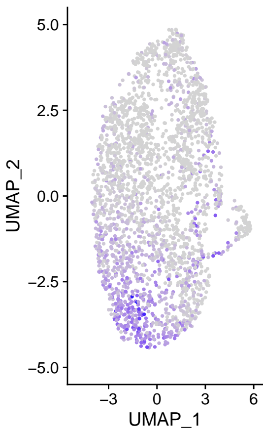
m_AC092069.1
