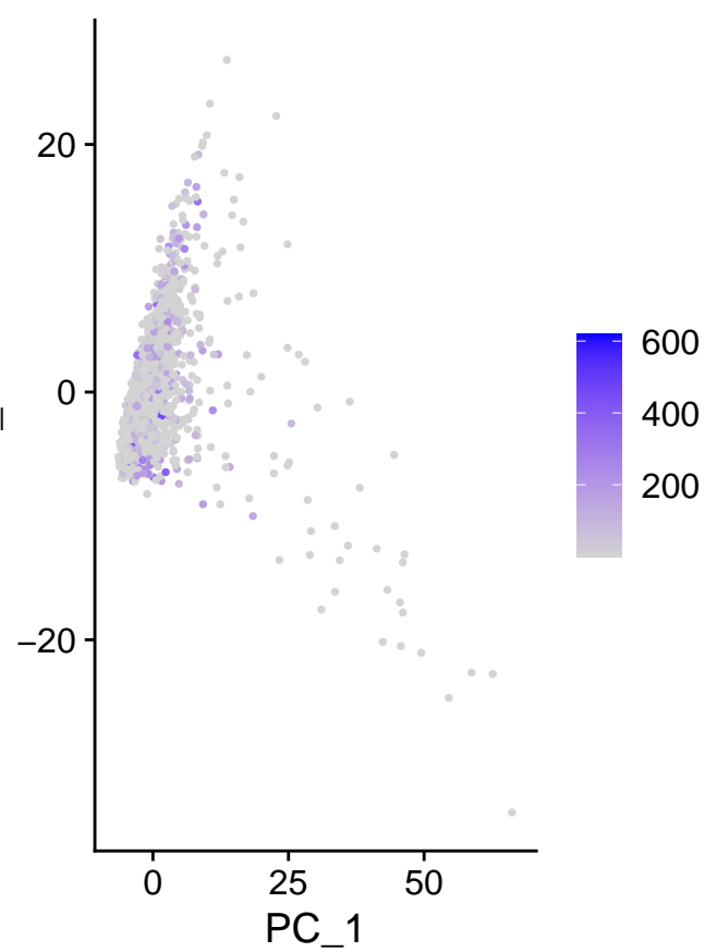
m_AC092069.1
