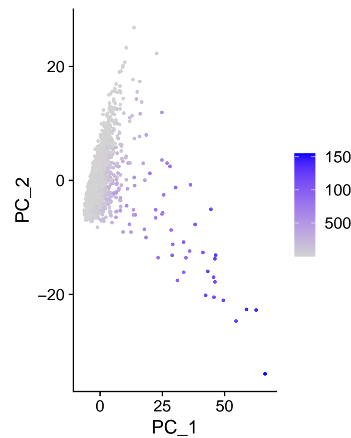
m_IGFBP7
