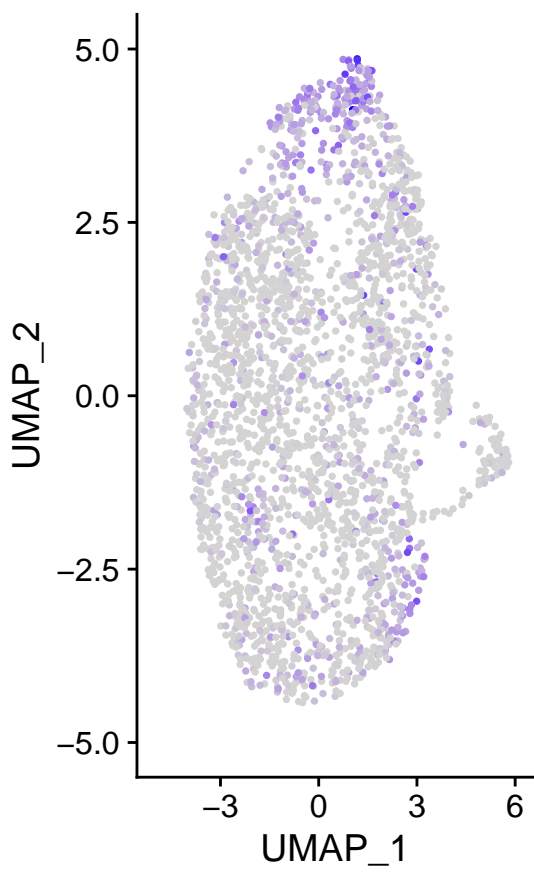
m_AC092069.1
