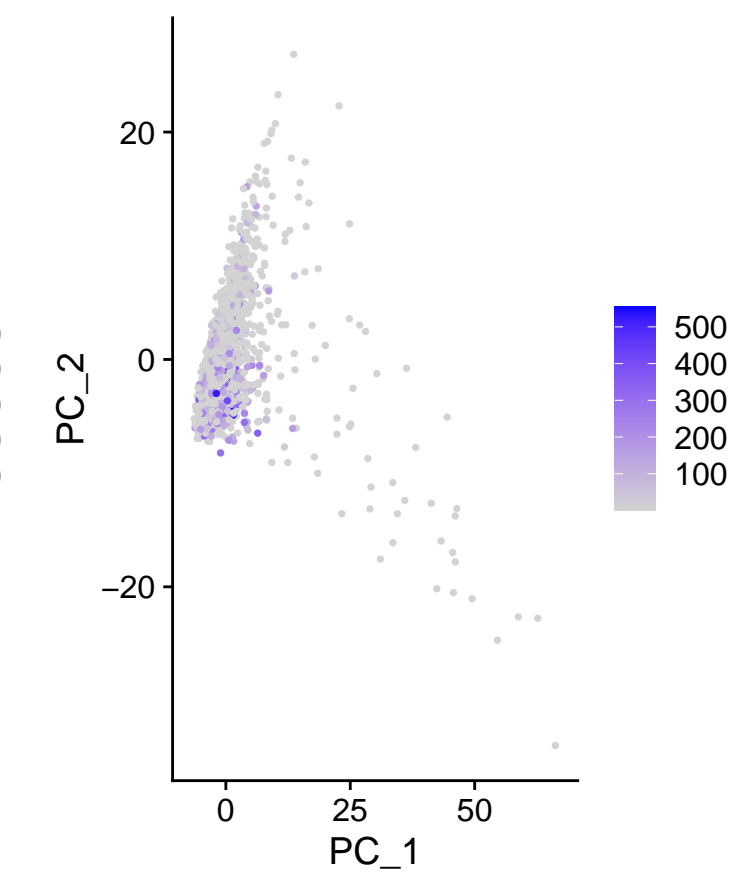
m_CD74
