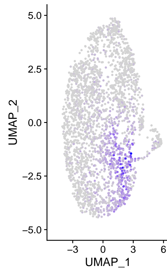
m_CD74
