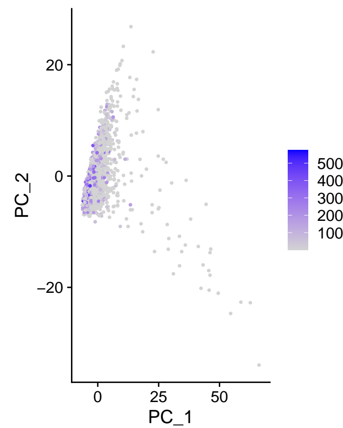
m_HAPLN2
