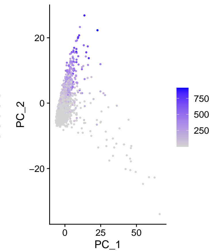
m_CD74
