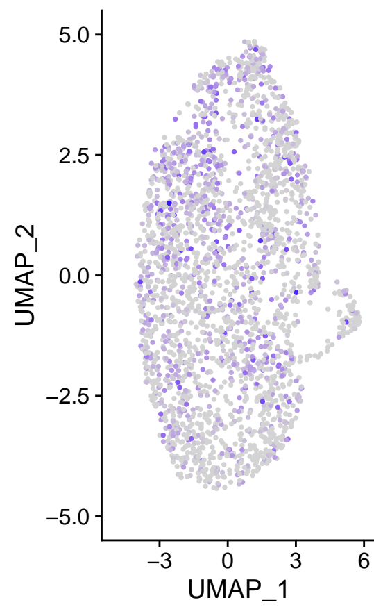
m_IGFBP7
