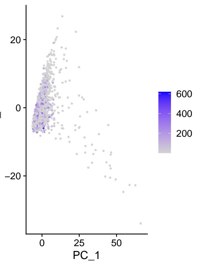
m_TPT1
