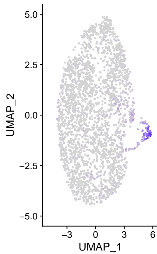
m_IGFBP7
