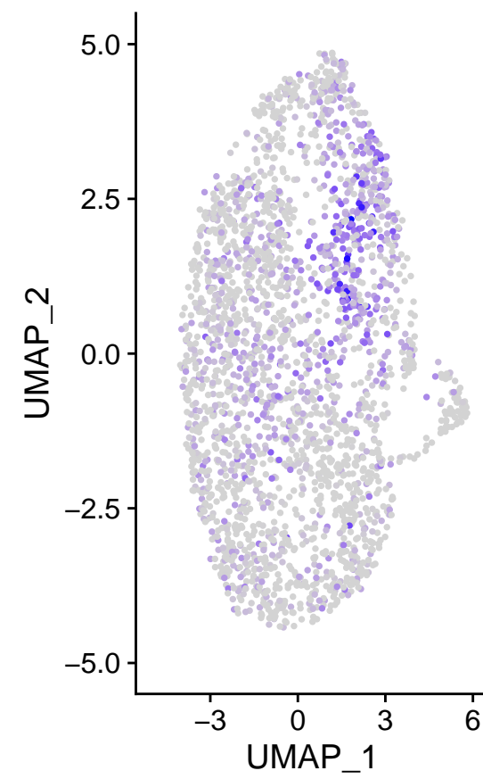
m_CD74
