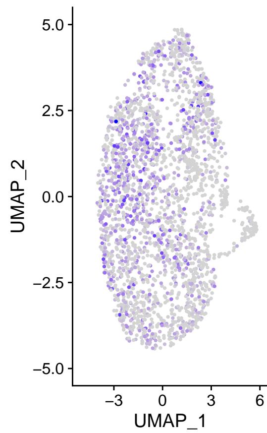
m_HAPLN2
