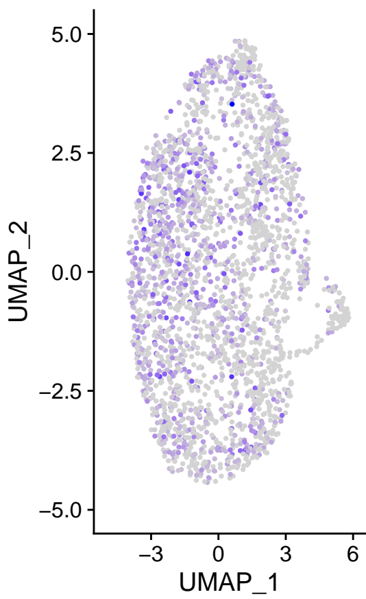
m_TPT1
