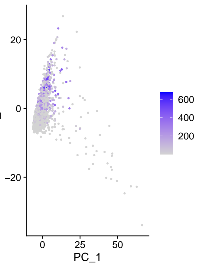
m_AC092069.1
