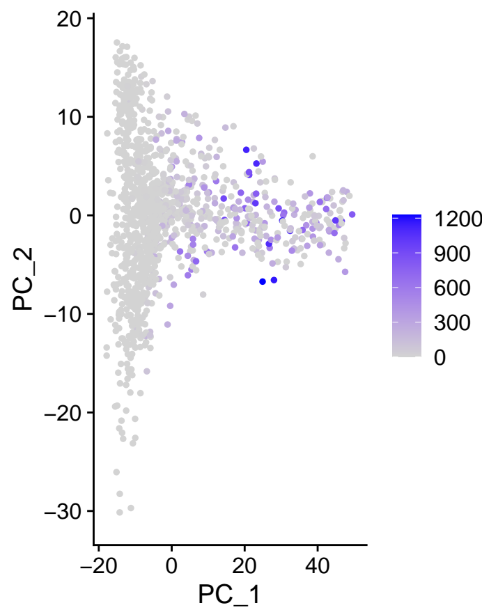
m_COX7C
