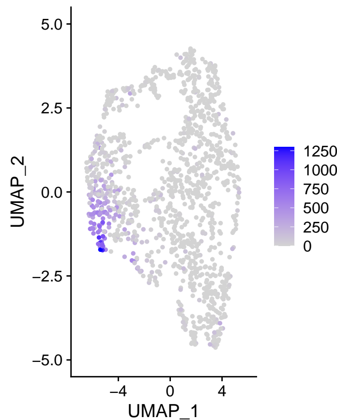
m_RBM6
