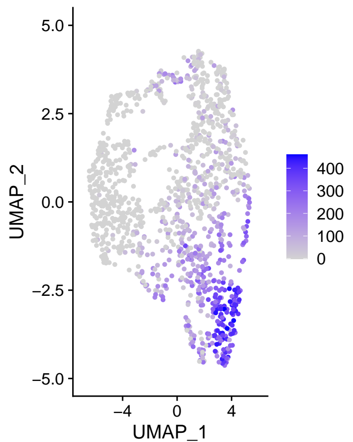
m_COX7C
