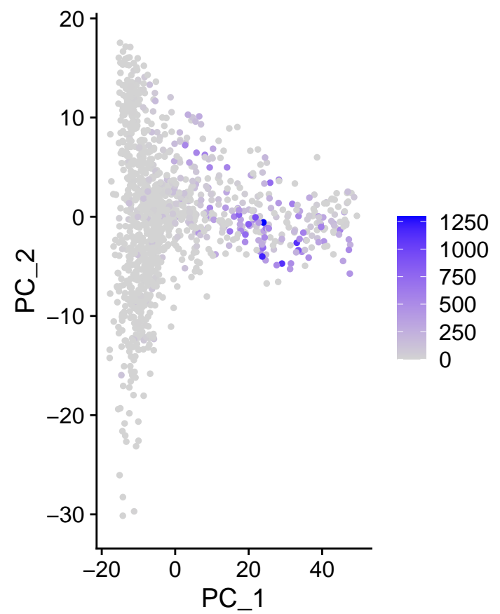
m_RBM6
