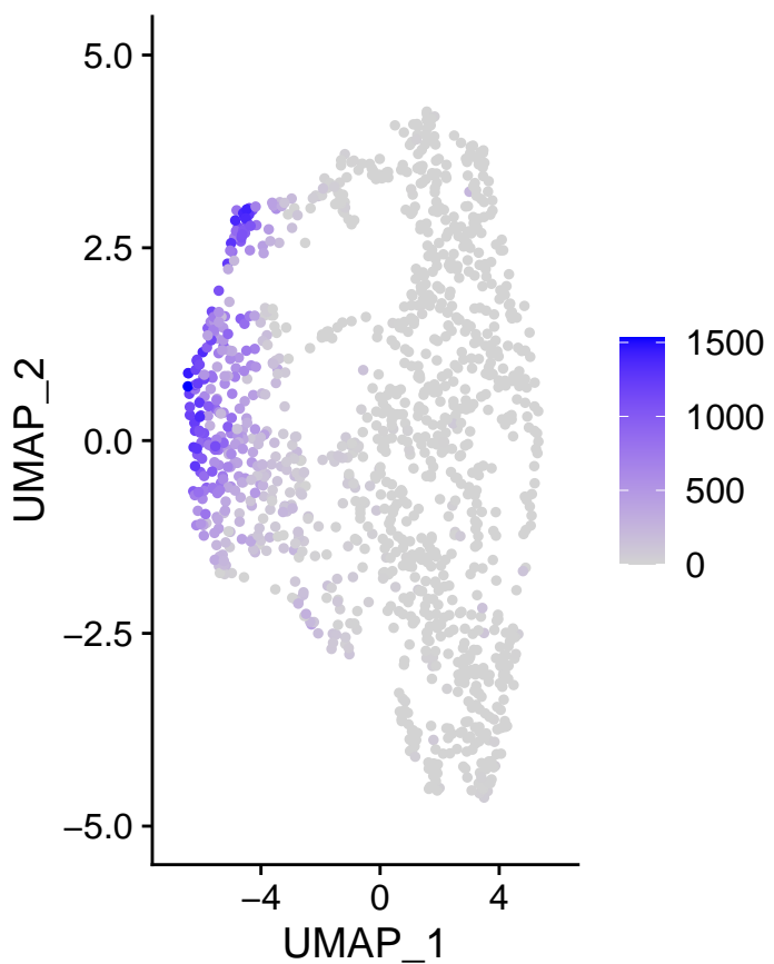
m_CACNA1A
