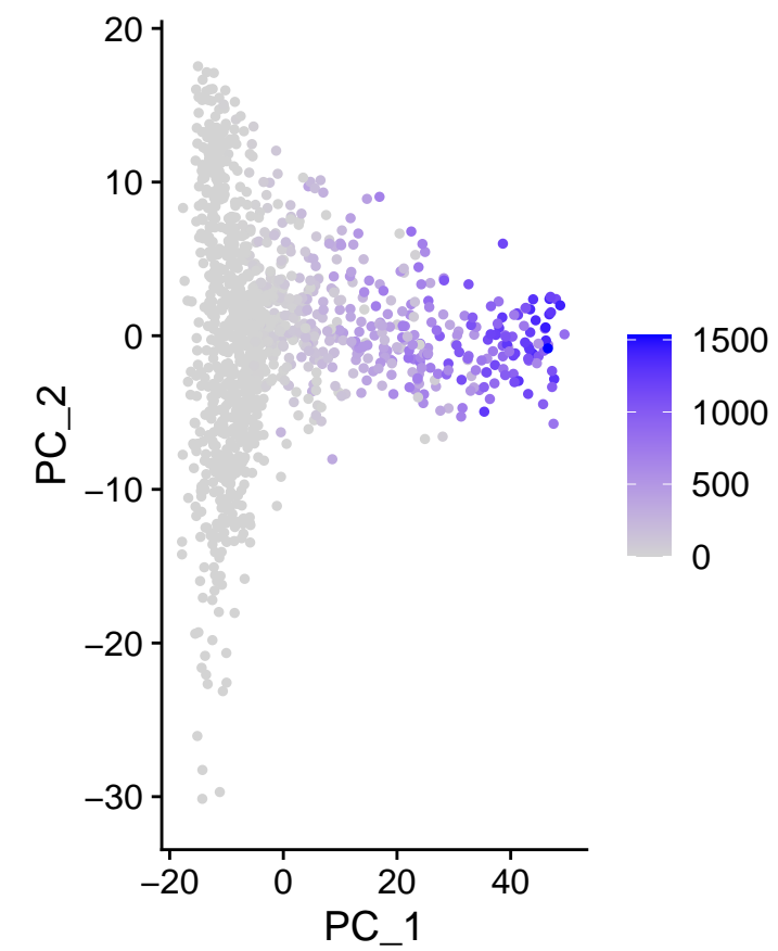
m_CACNA1A
