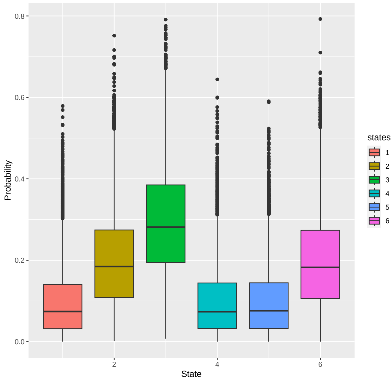
chr9-region_2684
