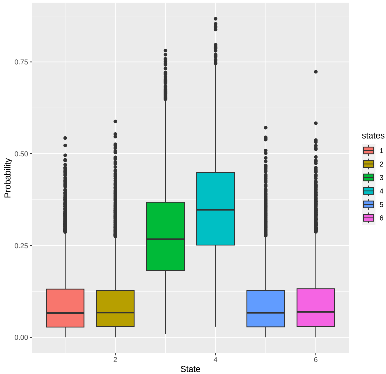
chr2-region_2886
