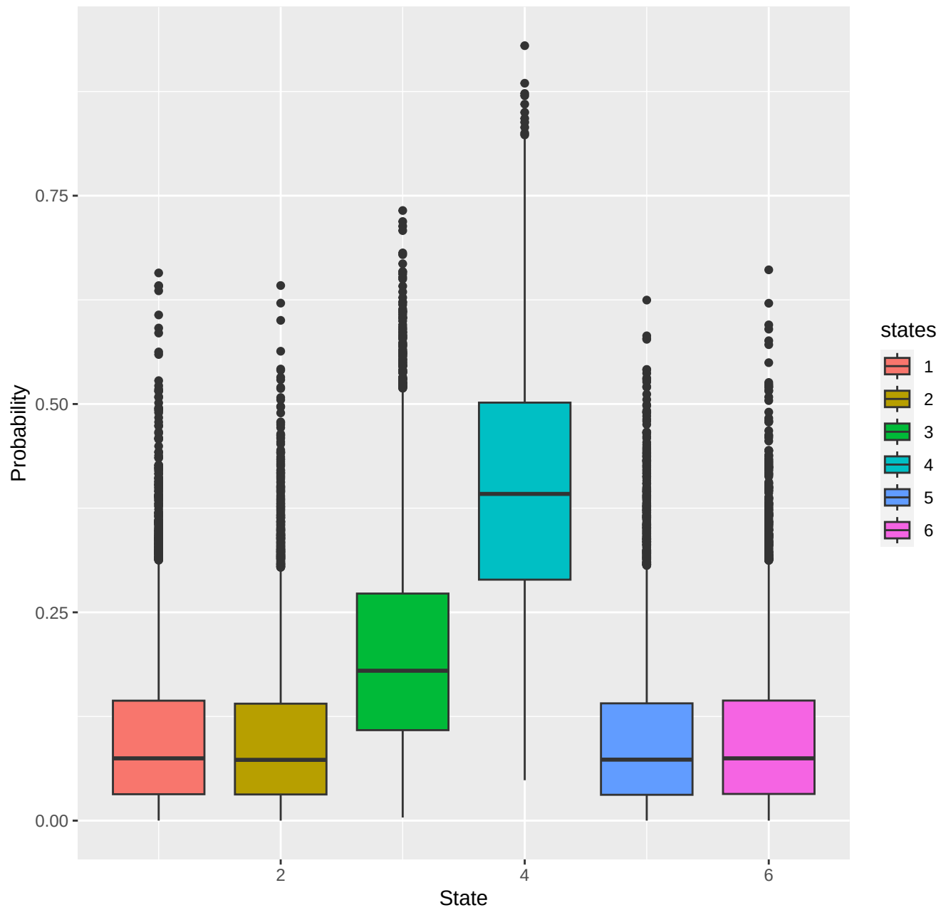
chr10-region_4733
