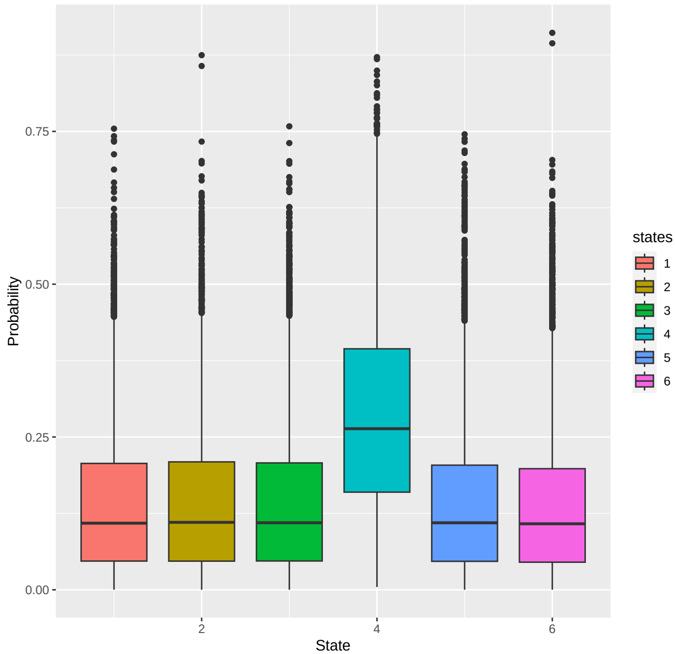
chr1-region_5119
