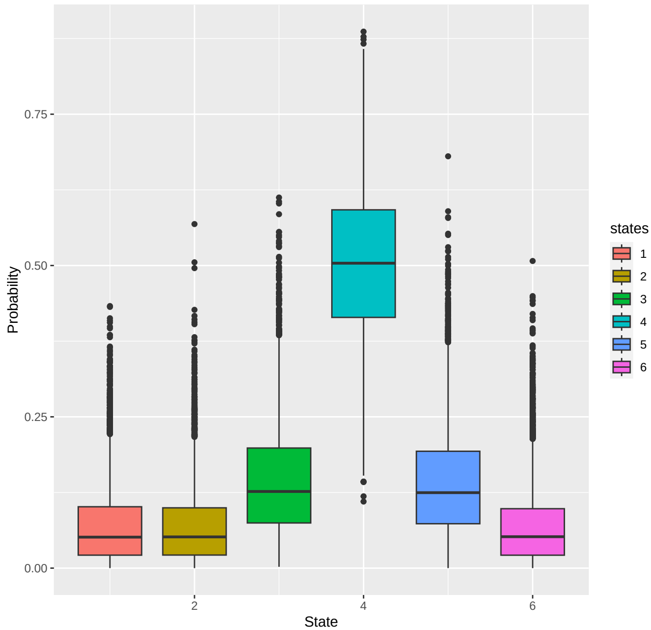
chr8-region_2098
