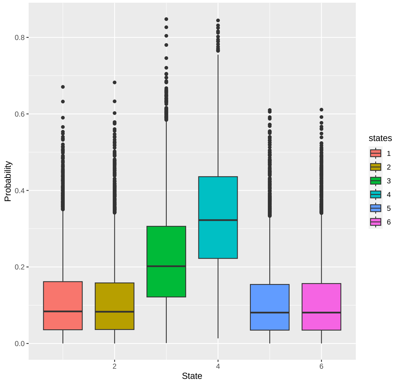
chr11-region_5497
