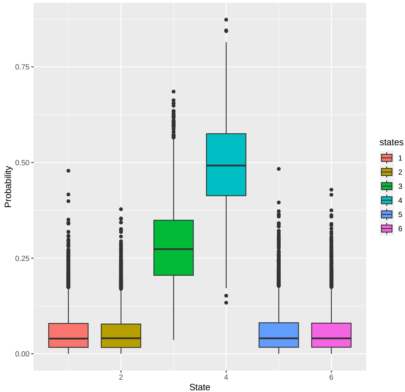
chr7-region_2444
