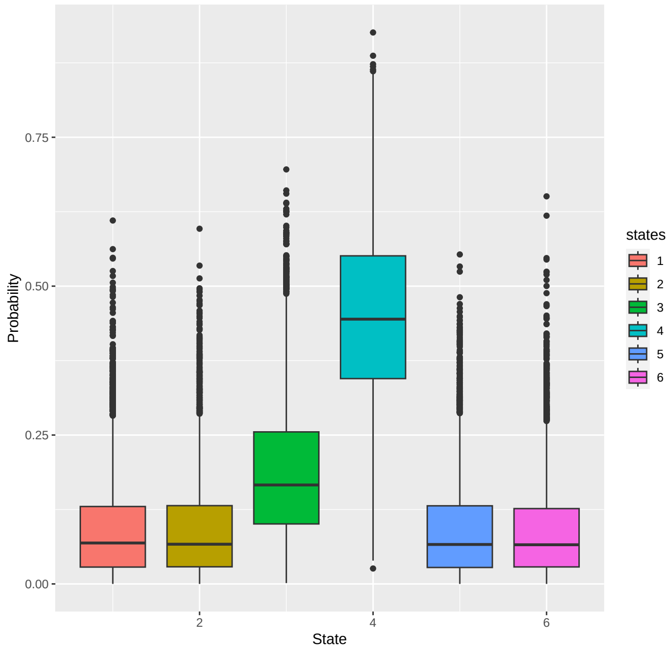
chr5-region_4218
