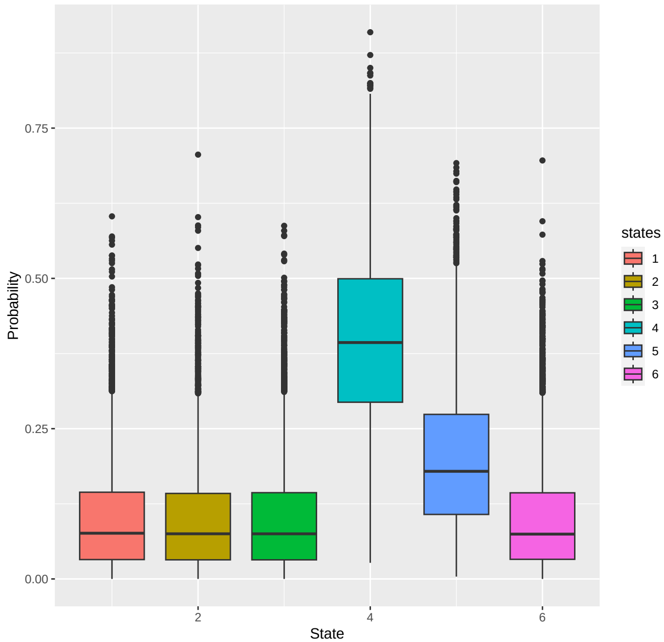
chr11-region_2689
