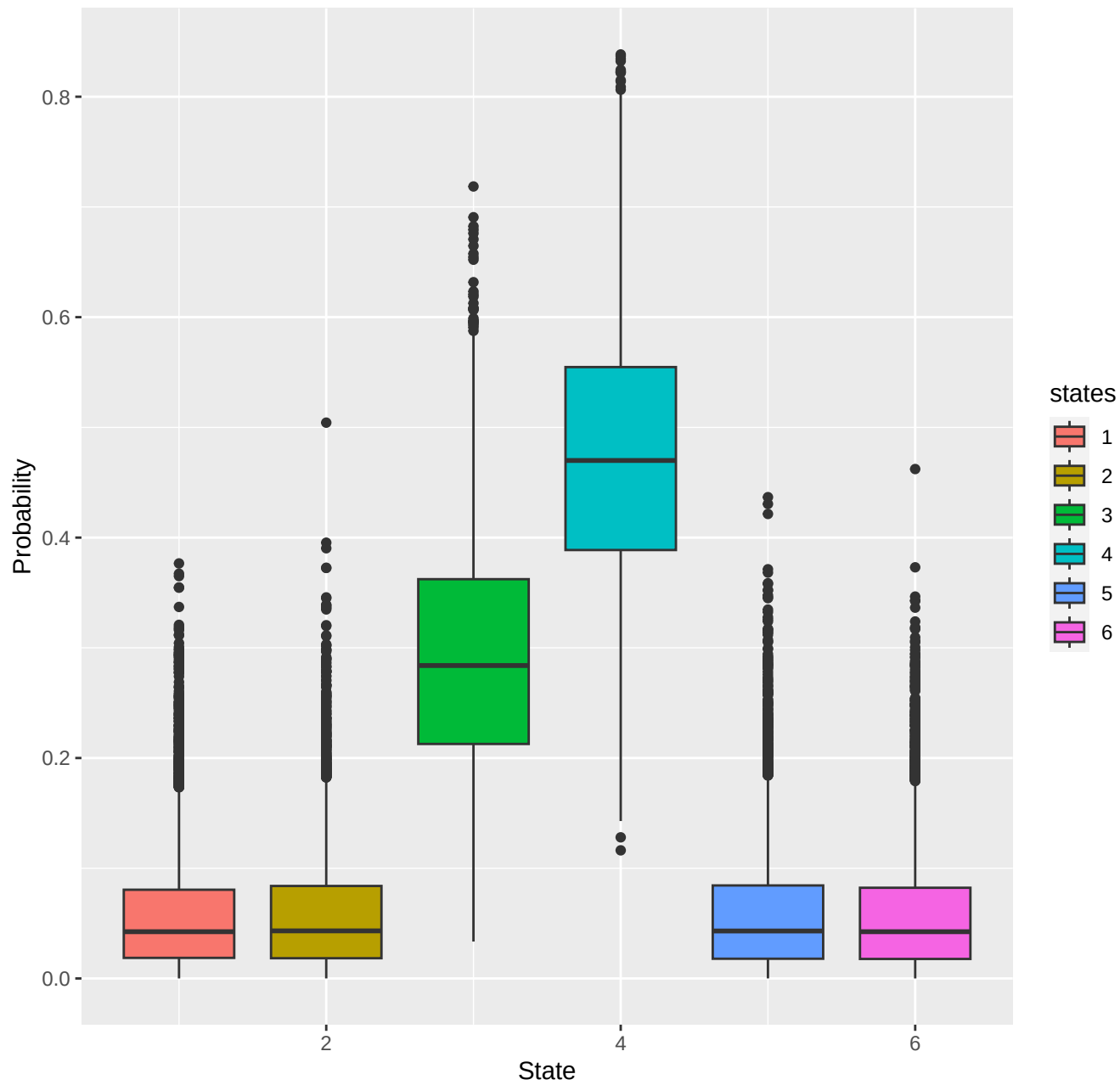
chr4-region_4013
