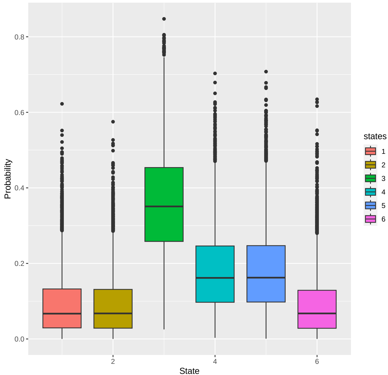
chr4-region_3754
