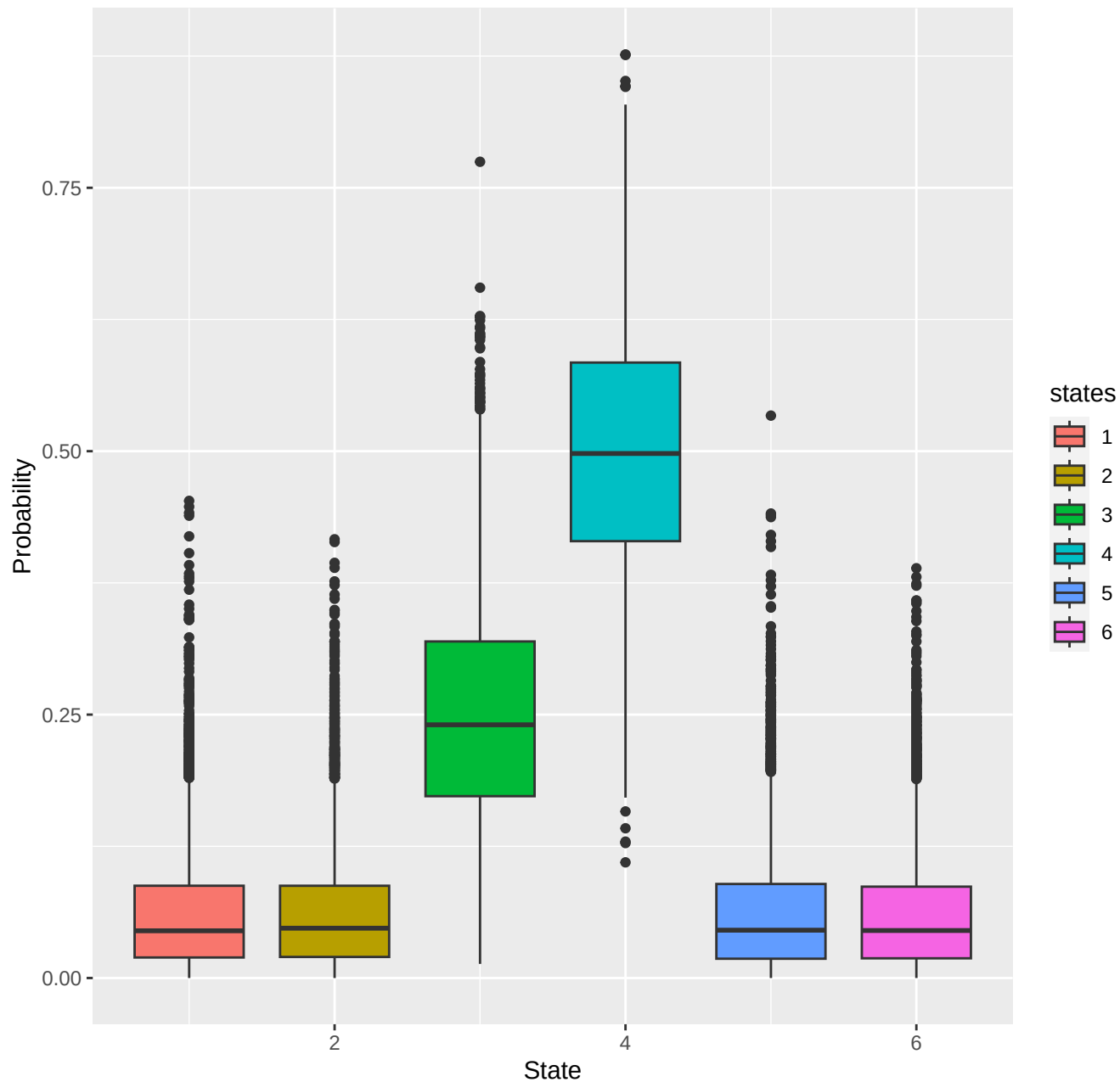
chr5-region_2807
