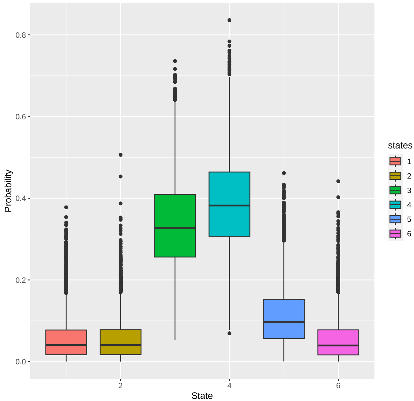
chr19-region_1856
