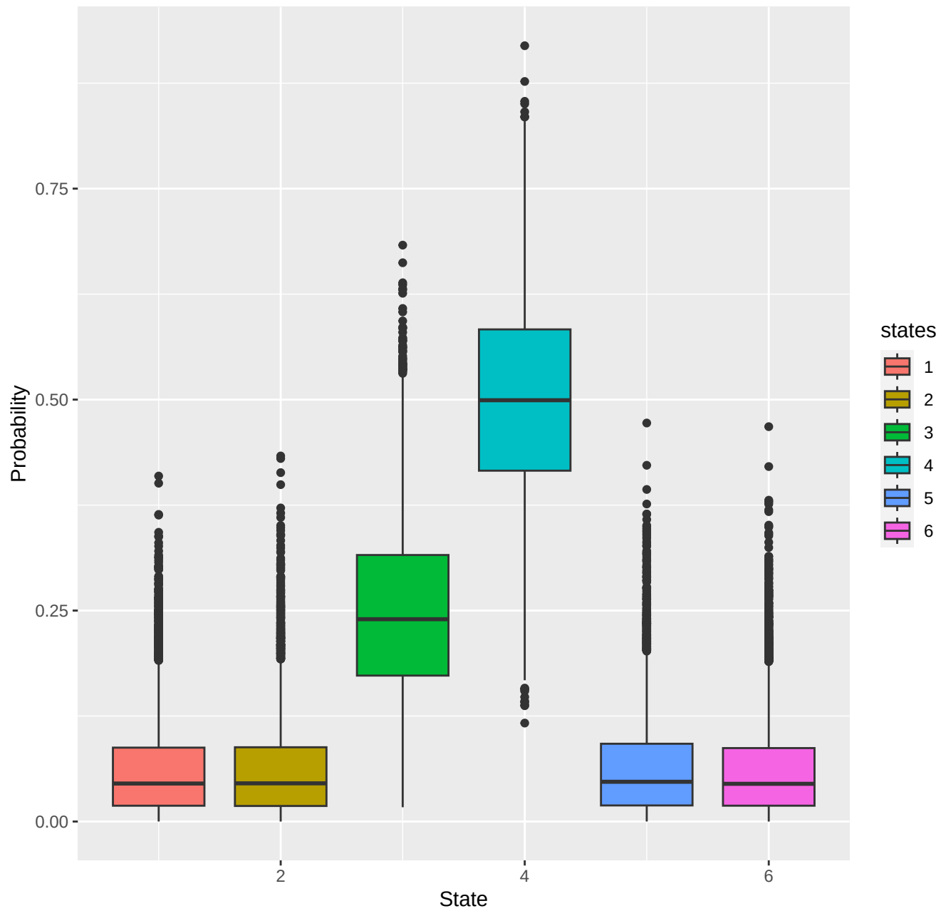
chr19-region_4358
