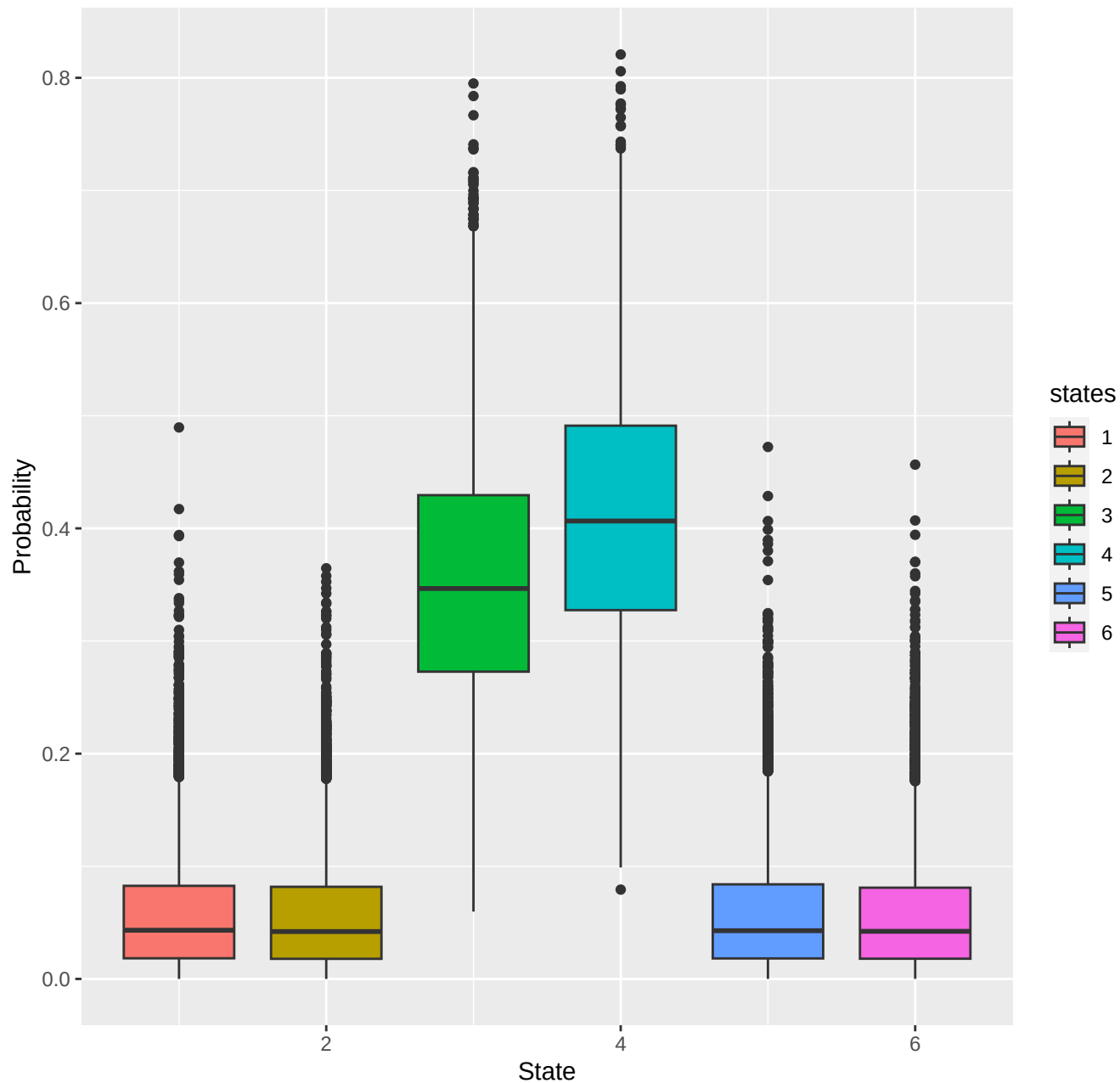
chr11-region_4022
