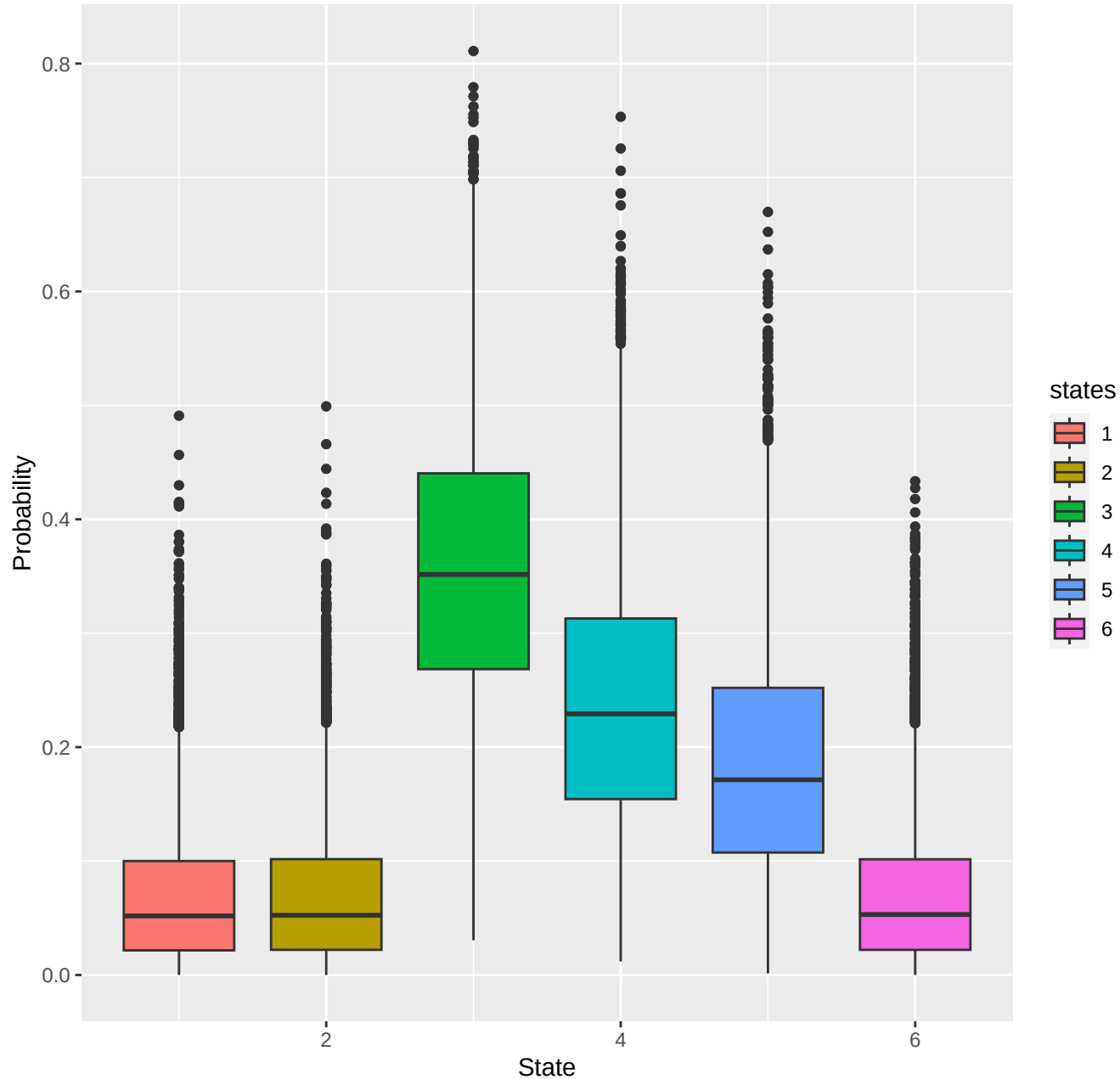
chr1-region_2959
