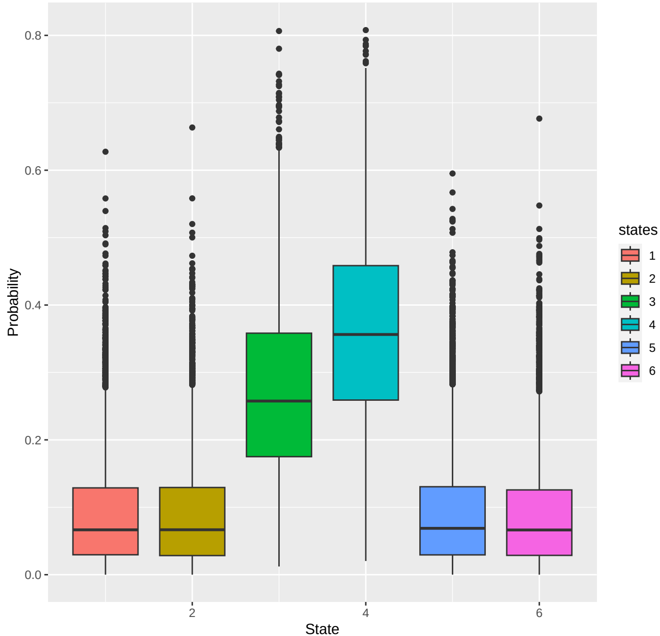
chr4-region_4215
