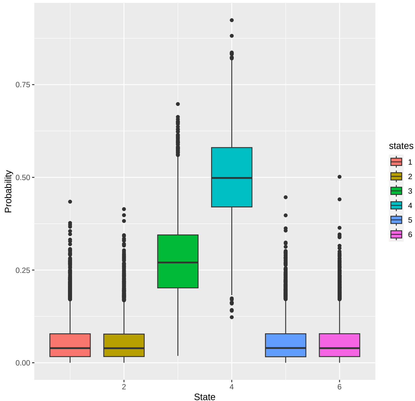
chr7-region_2392
