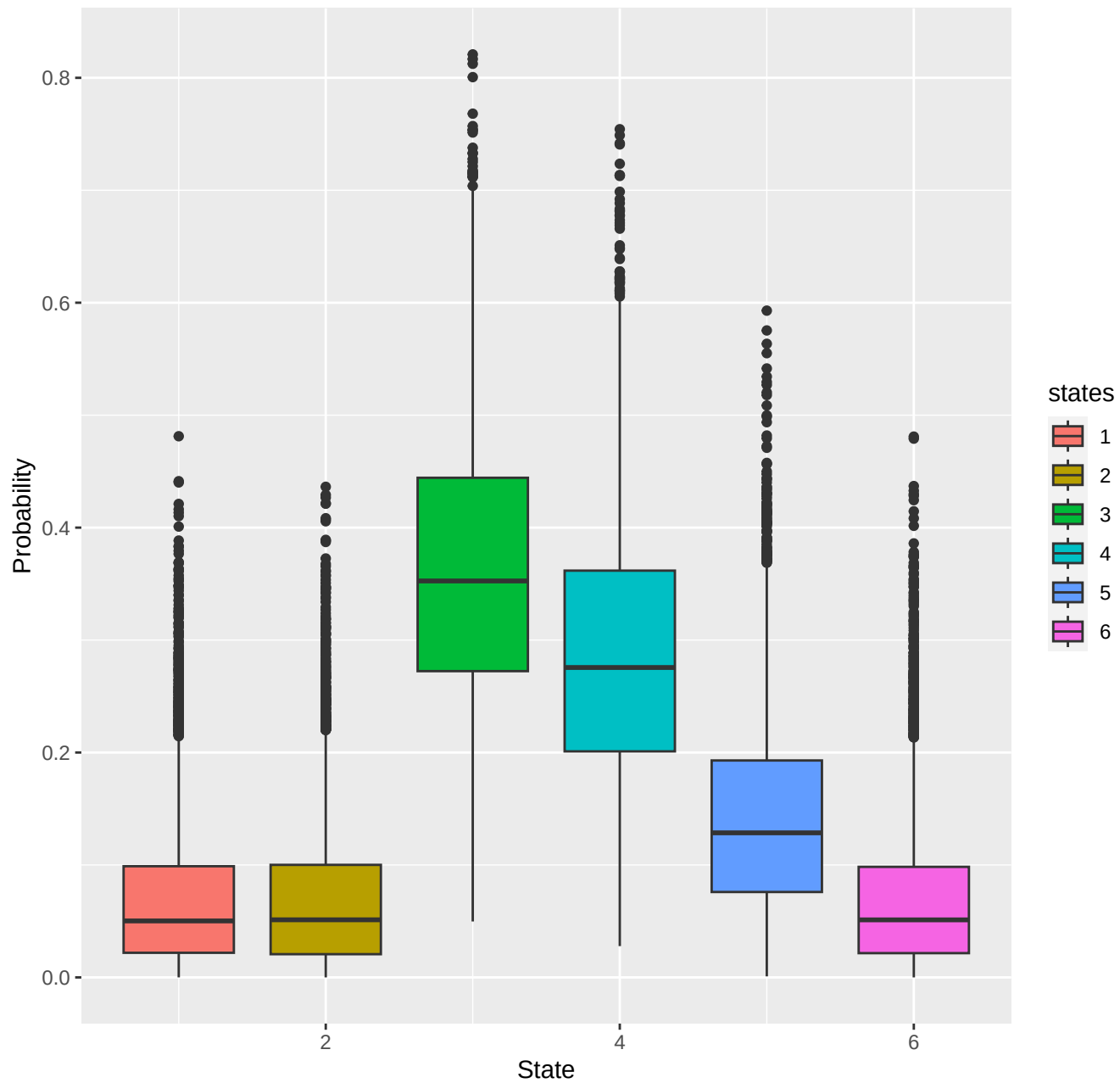
chr5-region_2006
