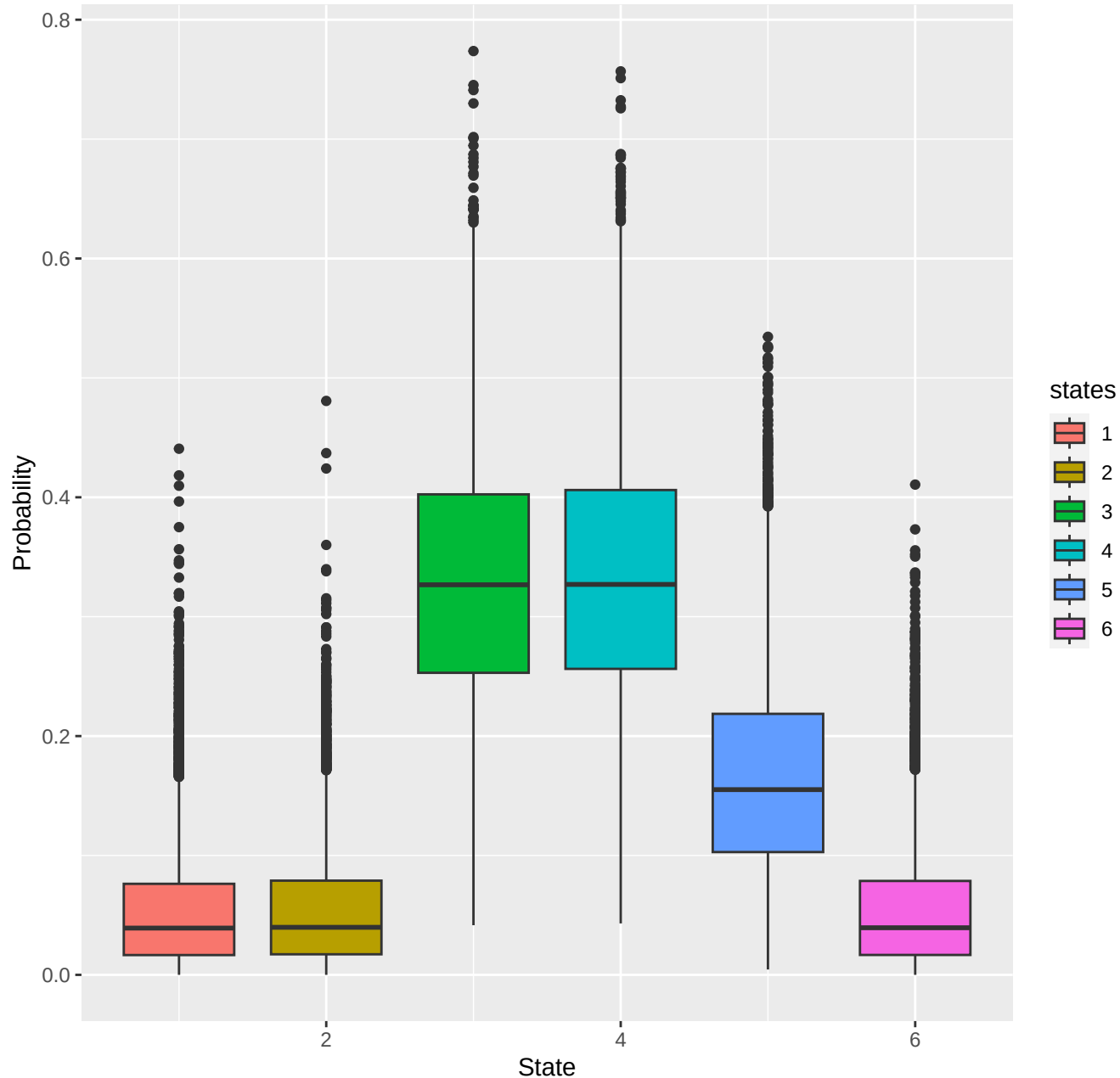
chr7-region_2062
