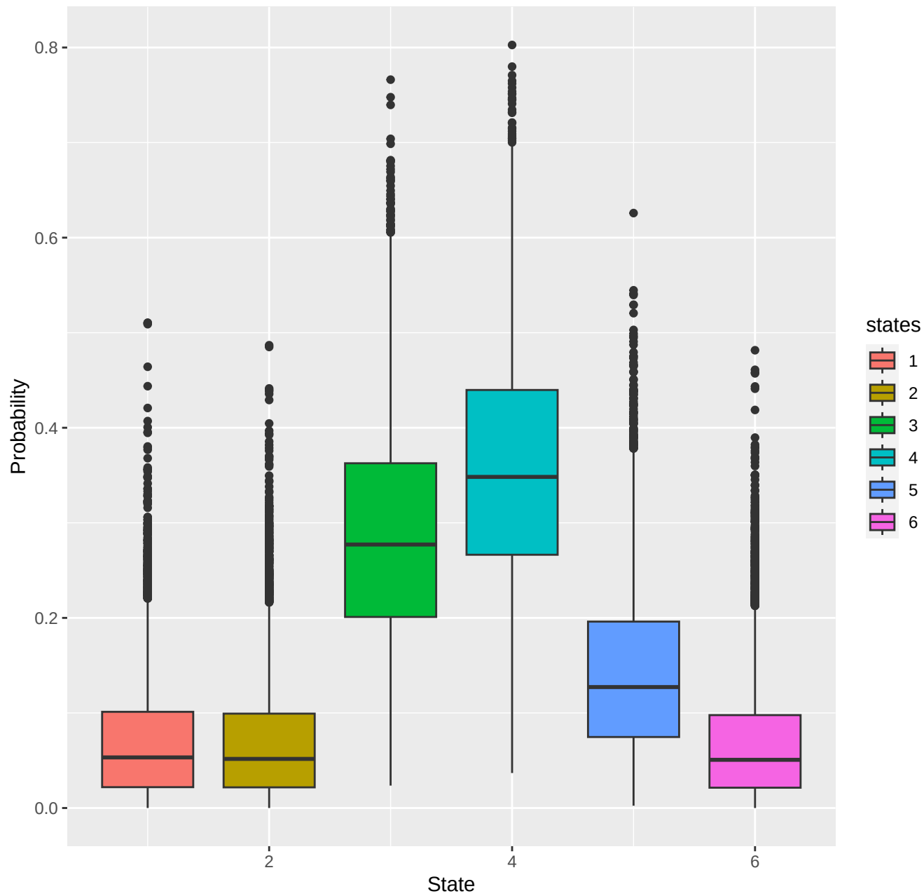
chr15-region_724
