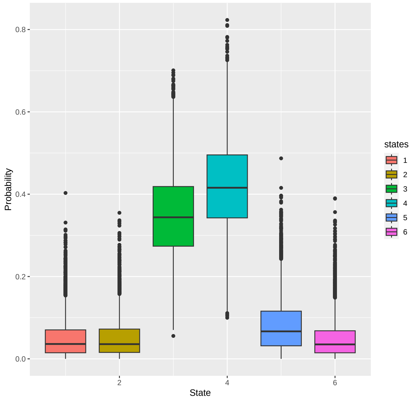
chr10-region_259
