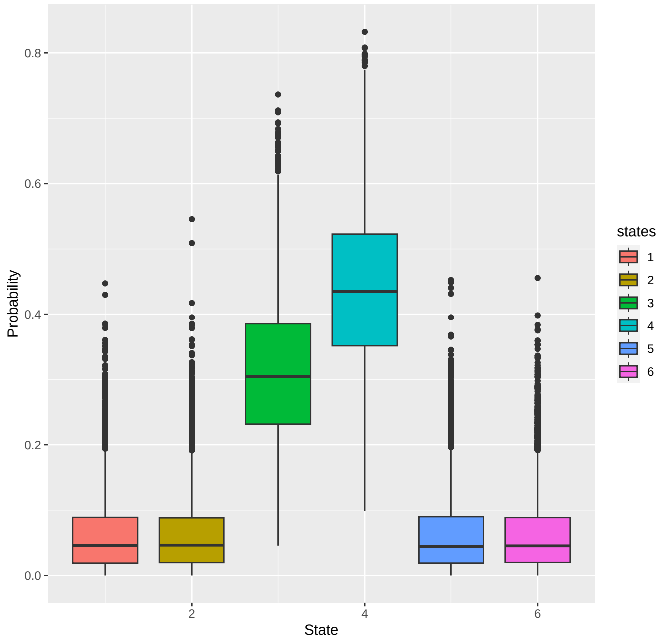
chr2-region_2306
