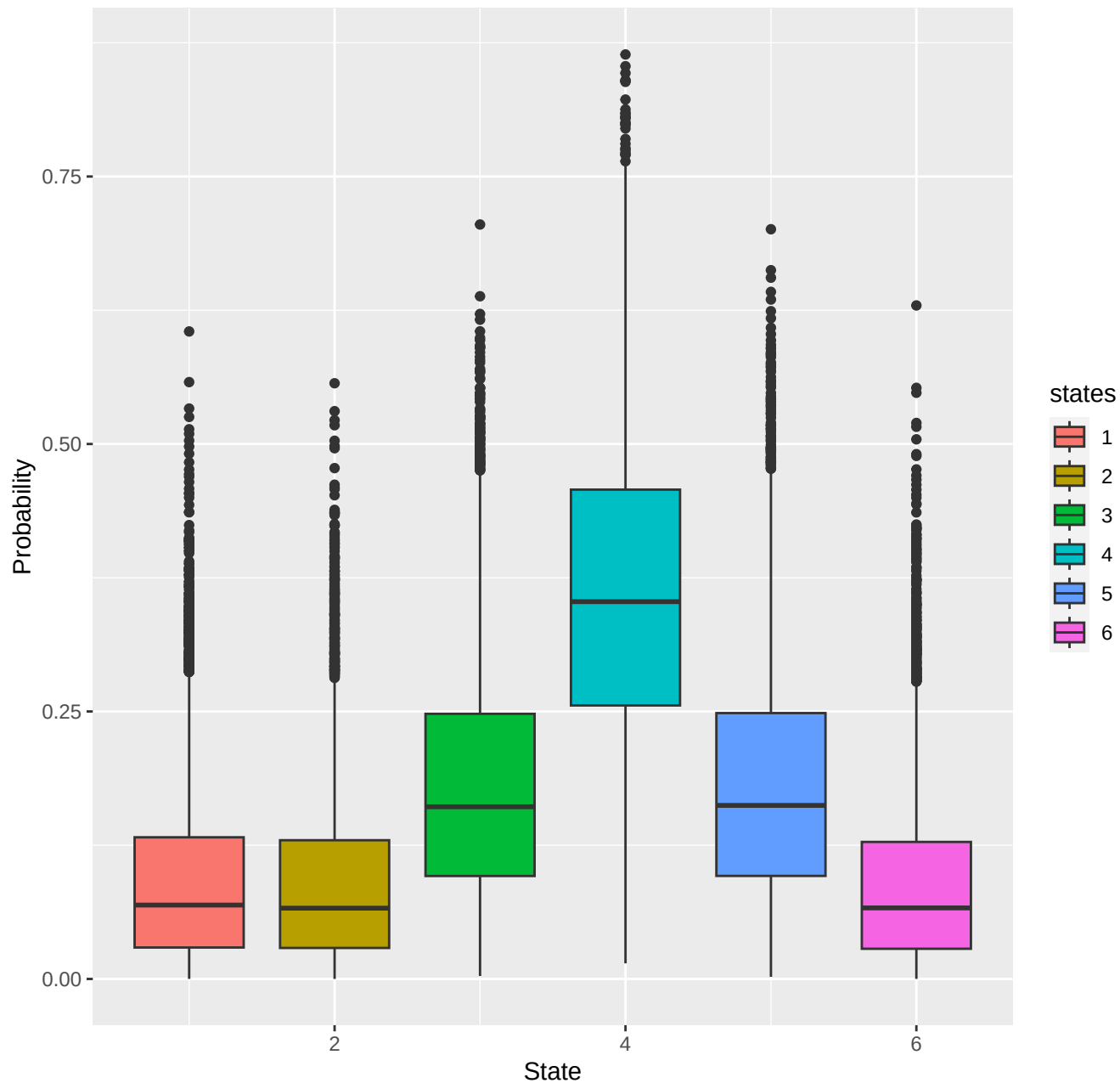
chr7-region_4221
