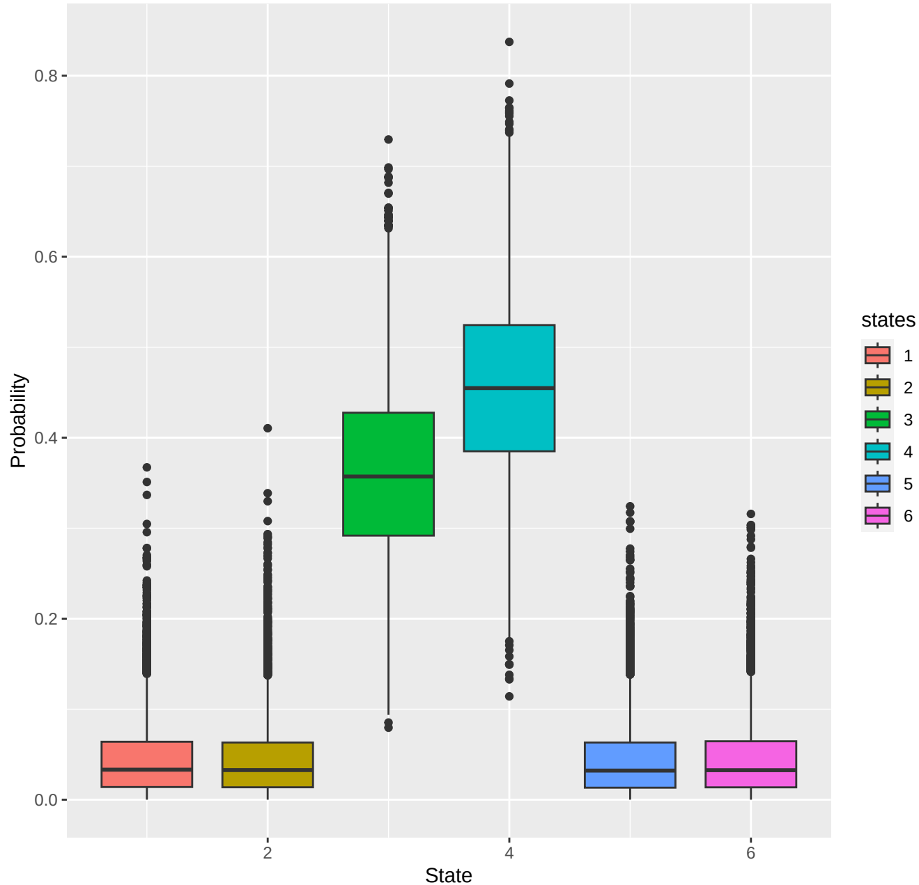
chr15-region_2501
