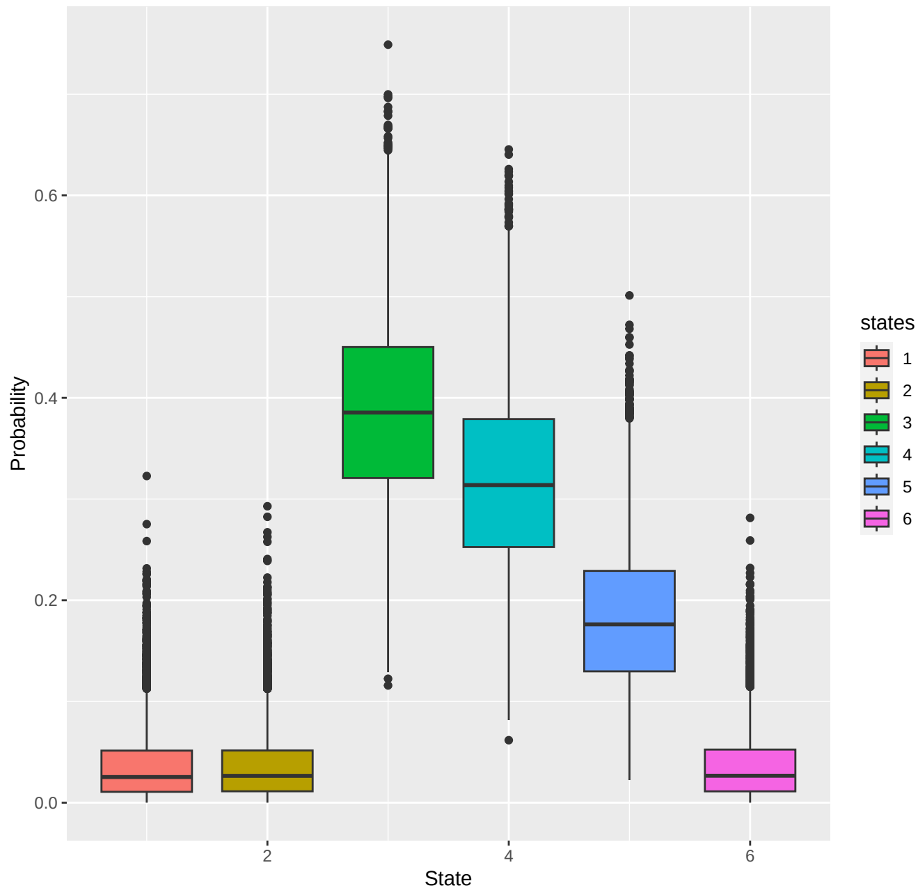
chr7-region_3267
