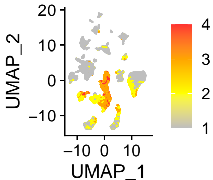
Squamous1
