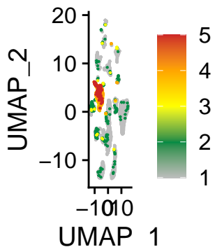
Monocytes5
