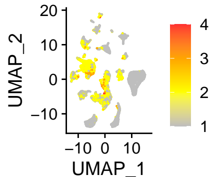
Interferon1
