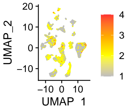
Hypoxia_UCell
