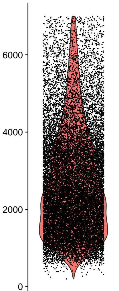
nFeature_RNA
