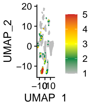
Ovarian.stroma6
