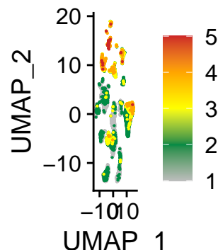
Epithelial12
