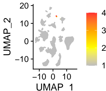
Ciliated_UCell
