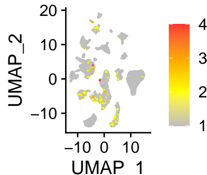
Metal_response_UCell
