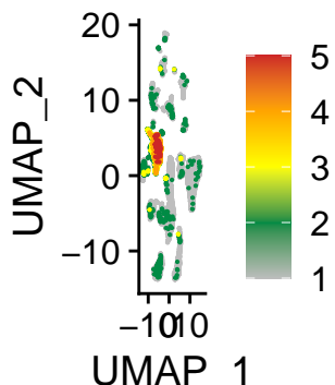
Macrophage10
