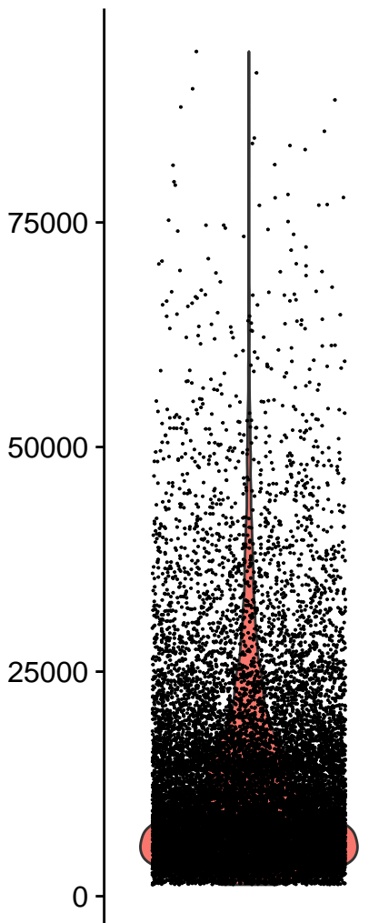
nCount_RNA
