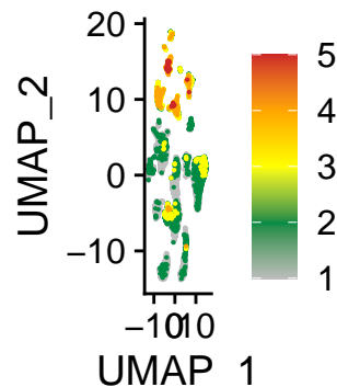
Epithelial.cancer8
