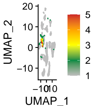
Ovarian.stroma6
